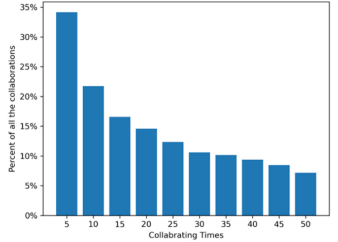
Fig. 4. Cumulative distribution of cooperating frequency of API pairs.
