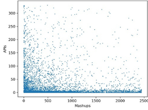
(a) The original mashup-API matrix
