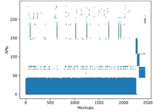
(b) The newly added APIs iterated over 20 times based on the recommender system
