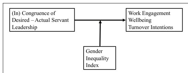
Figure 1. Conceptual model.
