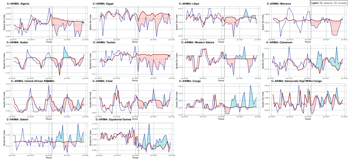
Figure C.4: C-ARIMA Northern African and Central African Countries
