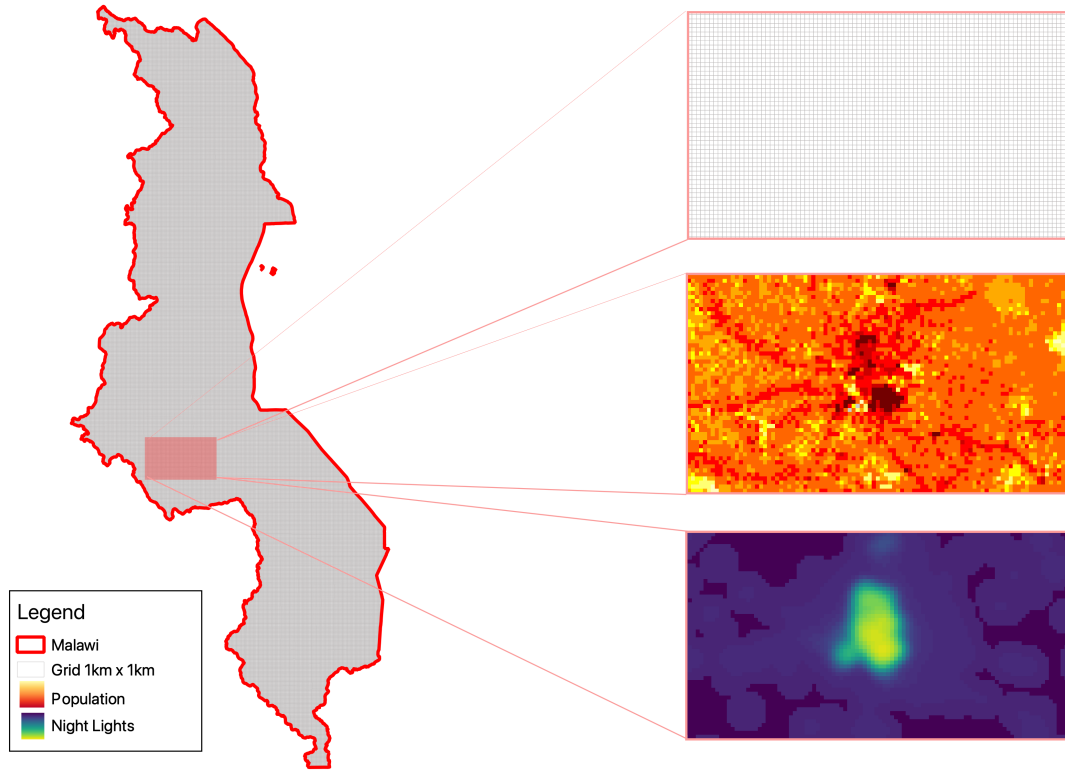
Figure 1: Construction of the 1km x 1km Grid and Aggregation of NTLs and Population data
