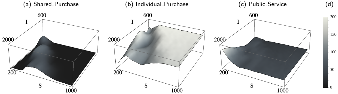
Figure 7: Impact of unit prices on the number of consumers in coalition
