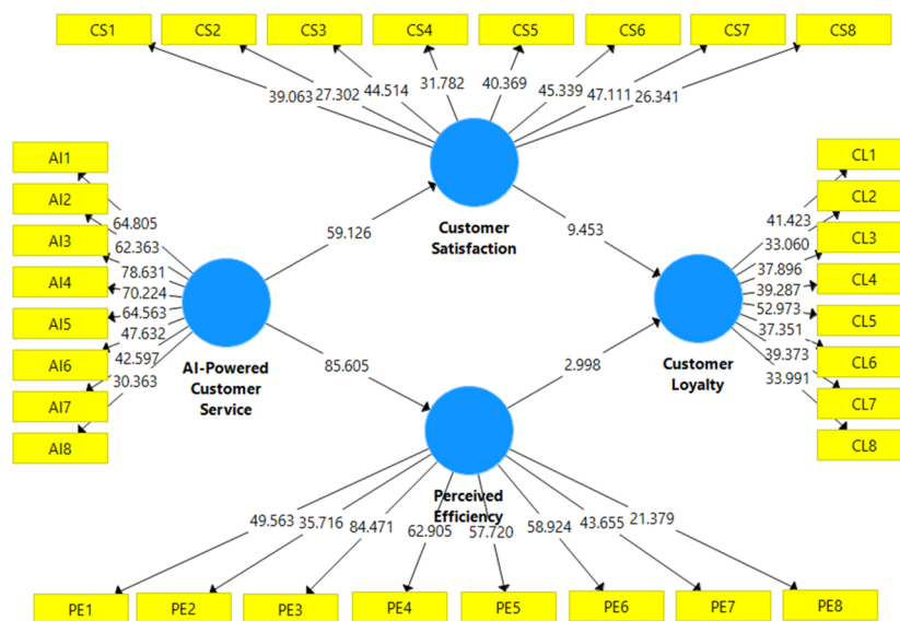
Figure 2. Structured model. Source: SMART-PLS calculation.
