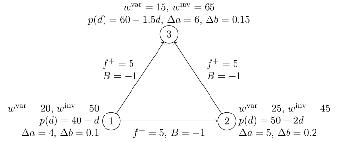
Fig. 2. 3-node network with the technical, economic, and uncertainty data used in the computational study.
