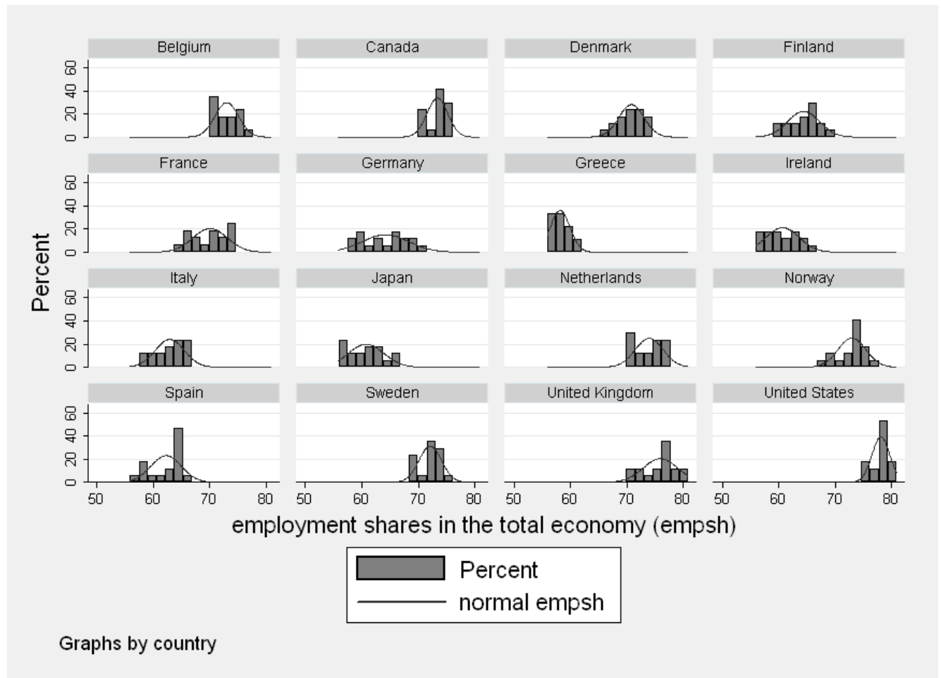
Figure A3 Industry Size distributions (as measured by employment share relative to total employment in the whole economy)
