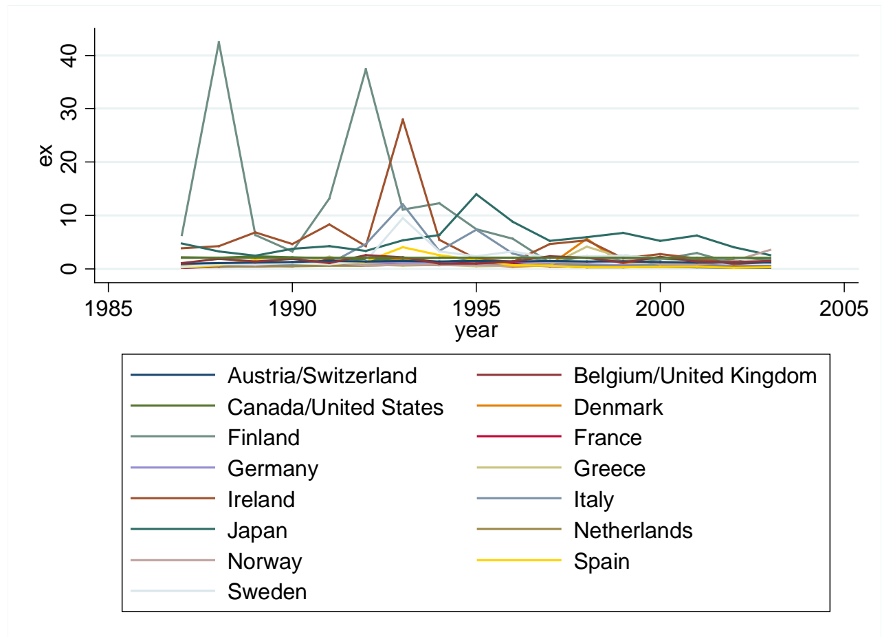
Figure 1 – Conditional Real Exchange Rate Volatility in OECD Countries, 1987 - 2003
