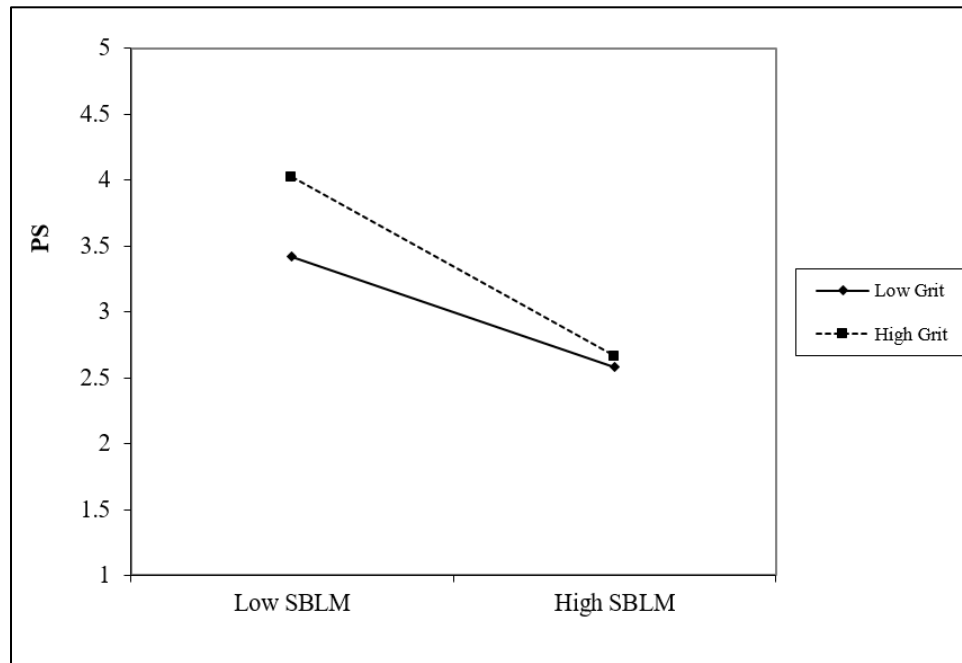
Figure 2: Moderation Graph
