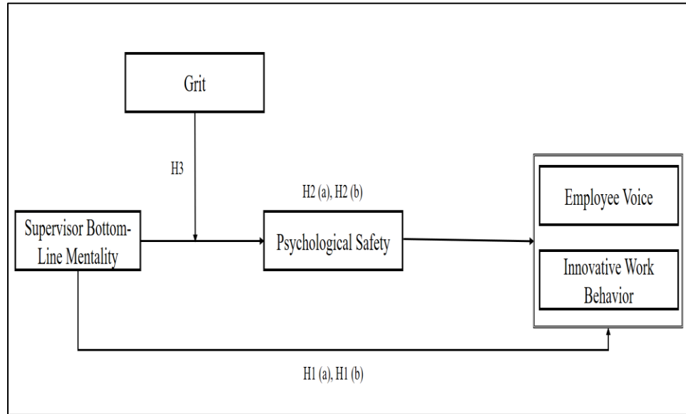
Figure 1: Hypothesized Model
