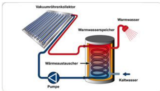
Solar thermal system
