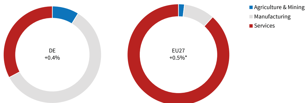
Figure 13: Change in the Level of Value Added after a 10% Reduction in Barriers
