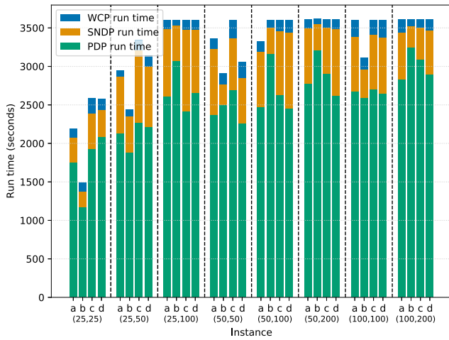
Fig. 8. The run time of the solution algorithm.
