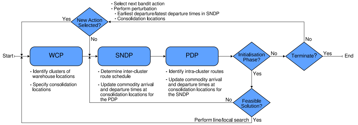
Fig. 5. The SCSNDP solution algorithm.
