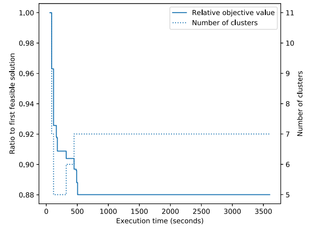
(b) (100, 100, 1) – Instance 4
