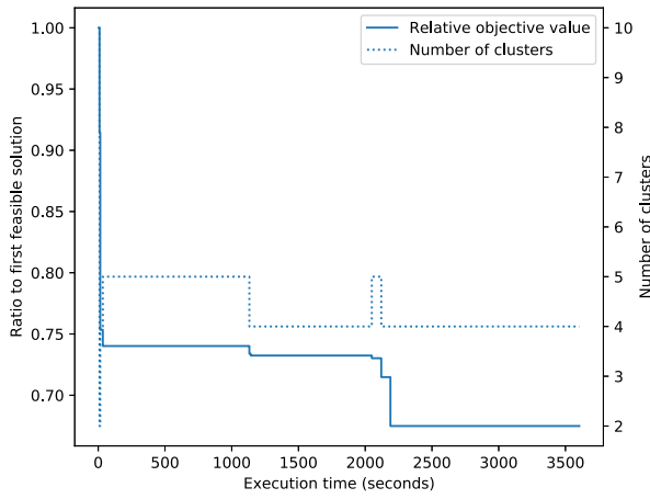
(a) (25, 100, 10) – Instance 1
