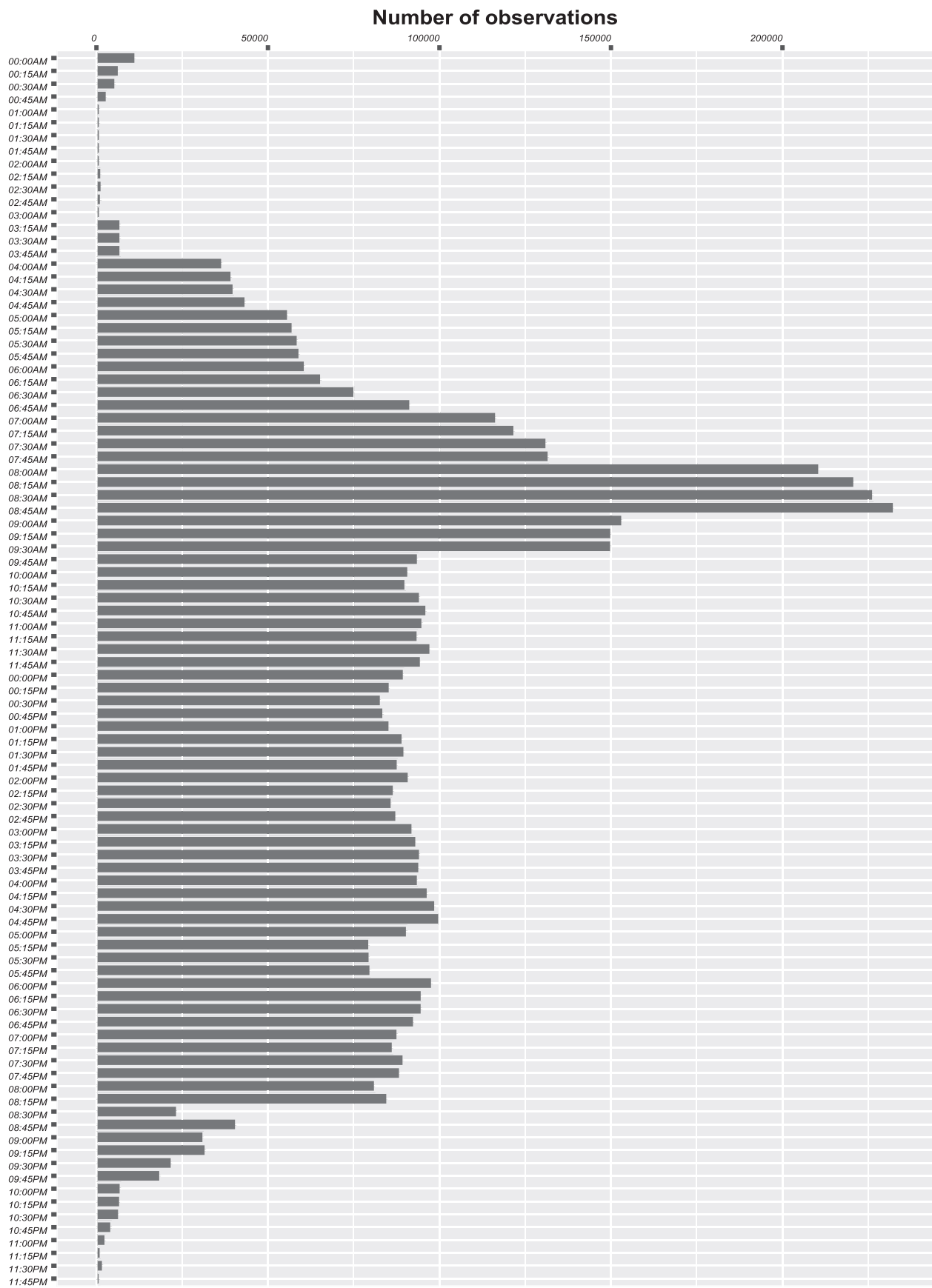
Fig. 3. Number of observations per time interval of 15 min.
