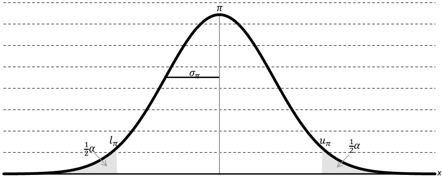
Figure 1: Symmetric confidence intervals of a normal distribution
