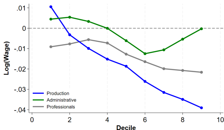
Figure 14: In Production, AI Compresses the Wage Distribution
