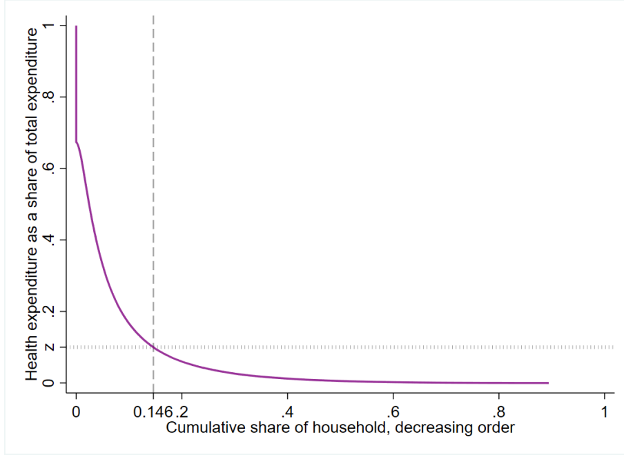
Figure 1: CDF
