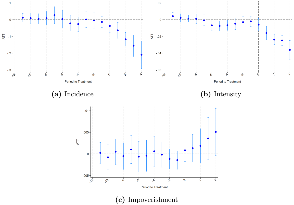
Figure 3: Event study
