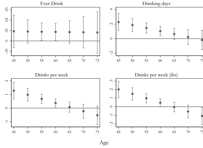
Figure 12: Heterogeneity: Age
