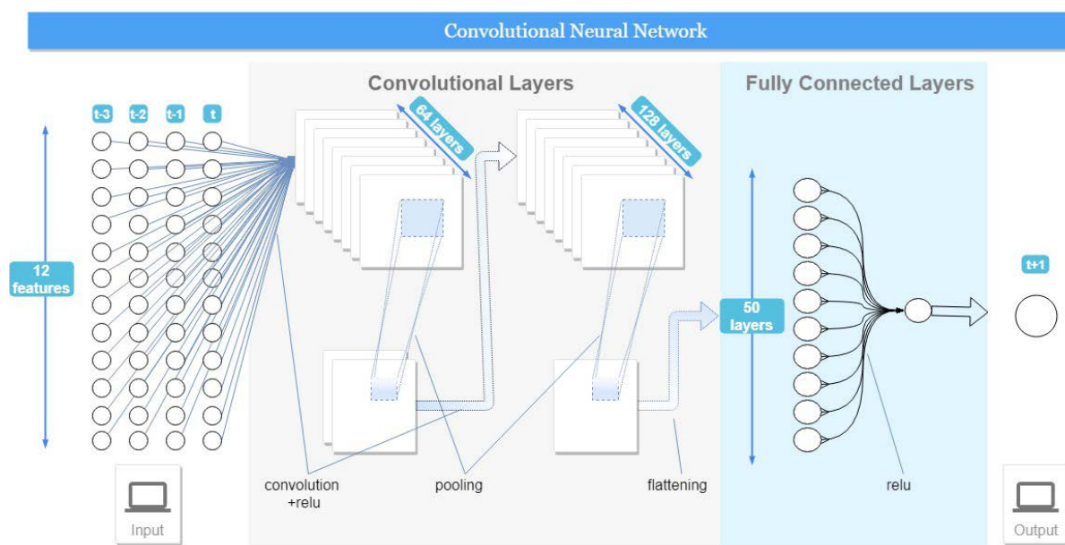
Fig. 3. Convolutional neural network architecture.
