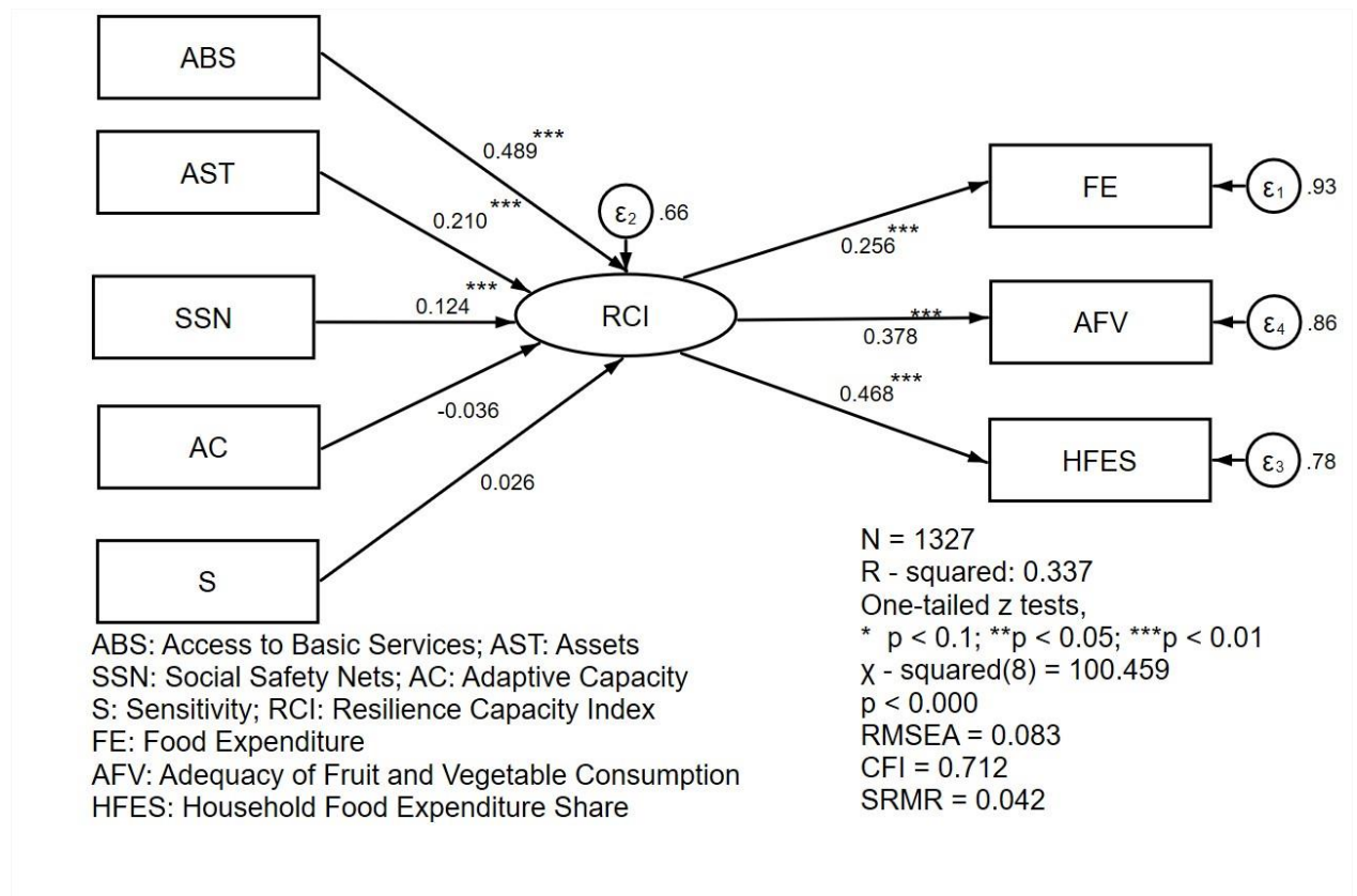
Figure 4.1 MIMIC Model
