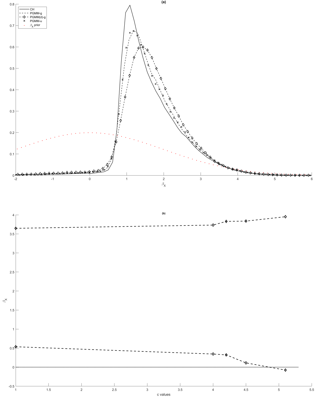
FIGURE 4. Upper panel (a): Linear IV (2) marginal (quasi-)posterior(s) for \beta_X and its marginal prior (red dotted curve); lower panel (b): Linear IV(2) 95% HPD intervals for \beta_X resulting from the PGMM approach along various priors for \mu , i.e., \mathcal{N}(0, c\Sigma_T\Omega_d\Sigma_T^\top) for various values of c .
