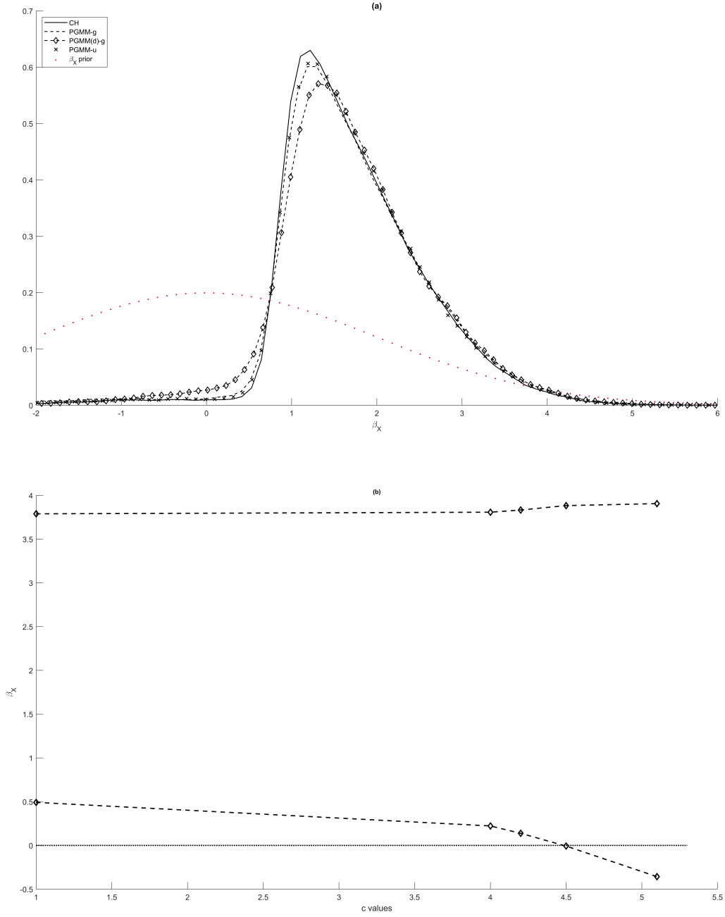
FIGURE 1. Upper panel (a): Linear IV (1) marginal (quasi-)posterior(s) for \beta_X and its marginal prior (red dotted curve). Lower panel (b): Linear IV(1) 95% HPD intervals for \beta_X resulting from the PGMM approach along various priors for \mu , i.e., \mathcal{N}(0, c\Sigma_T\Omega_d\Sigma_T^\top) for various values of c .
