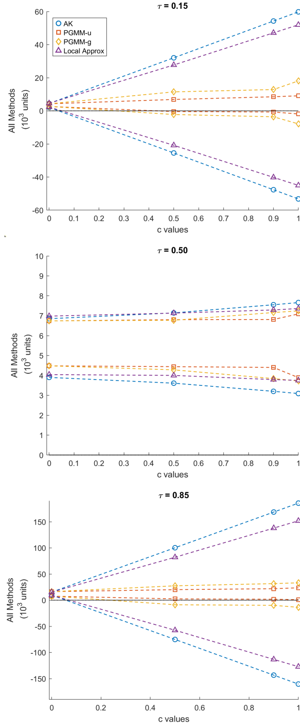
FIGURE 3. This figure shows the 95% intervals constructed for the treatment effect parameter, \beta_{X,\tau} , using the limiting approximation indicated by Theorem 1 (Local Approx), PGMM (PGMM-u denotes the cases with uniform priors on \mu while PGMM-g denotes the cases with Gaussian priors on \mu_\tau ) and AK (AK) for IVQR with \tau = 0.15, 0.50, 0.85 and c = 0, 0.5, 0.9, 1.0 .
