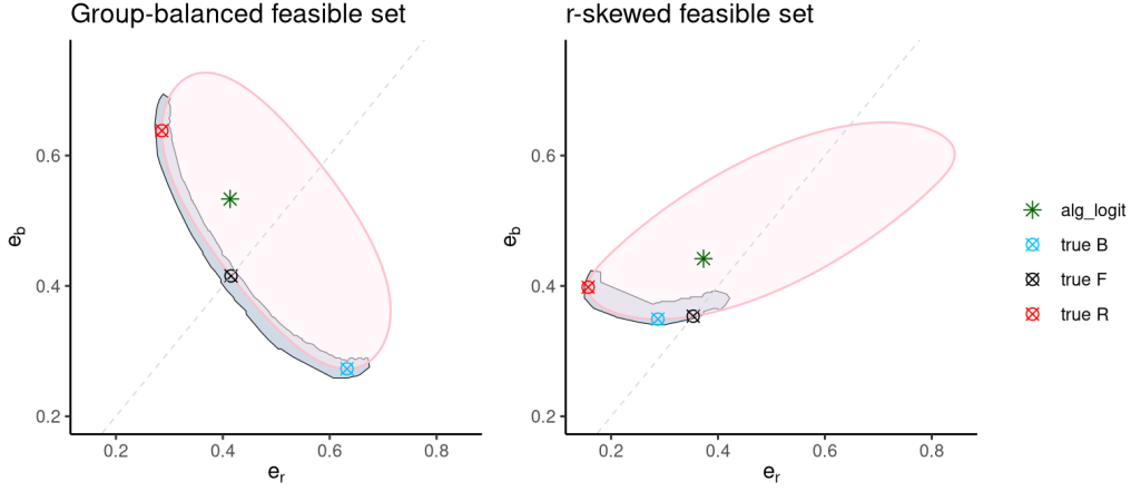
FIGURE 5.—True feasible set \mathcal{E} for group-balanced DGP (left) and r -skewed DGP (right), based on evaluating \mathcal{S}_{\mathcal{E}}(q) in Eq. (12) at true \theta in 500 directions, with expectations approximated by averaging over 10^7 observations drawn from the respective DGP. True R and B obtained similarly, using Eq. (13). True F based on evaluating Eq. (19) at true \theta and minimizing over c via stochastic gradient descent. True risk e^* (green asterisk) induced by the logit algorithm based Eq. (5). Shaded region: 95% confidence set for \mathcal{F} built using 10,000 observations drawn from the respective DGP and test inversion detailed in Section 5.2 with \Delta\theta estimated by logit lasso.
