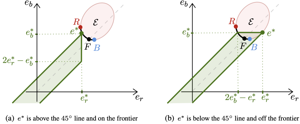
FIGURE 3.—The set \mathcal{C}(e^*) , which collects all improvements relative to e^* , is the region shaded in green. Its shape depends on whether e^* lies above or below the 45^\circ line. Panel (a) shows an example of the case where e^* lies on the frontier and there exists a hyperplane that properly separates \mathcal{C}(e^*) and \mathcal{E} , whereas in panel (b) e^* is not on the frontier and no hyperplane can separate \mathcal{C}(e^*) and \mathcal{E} .
