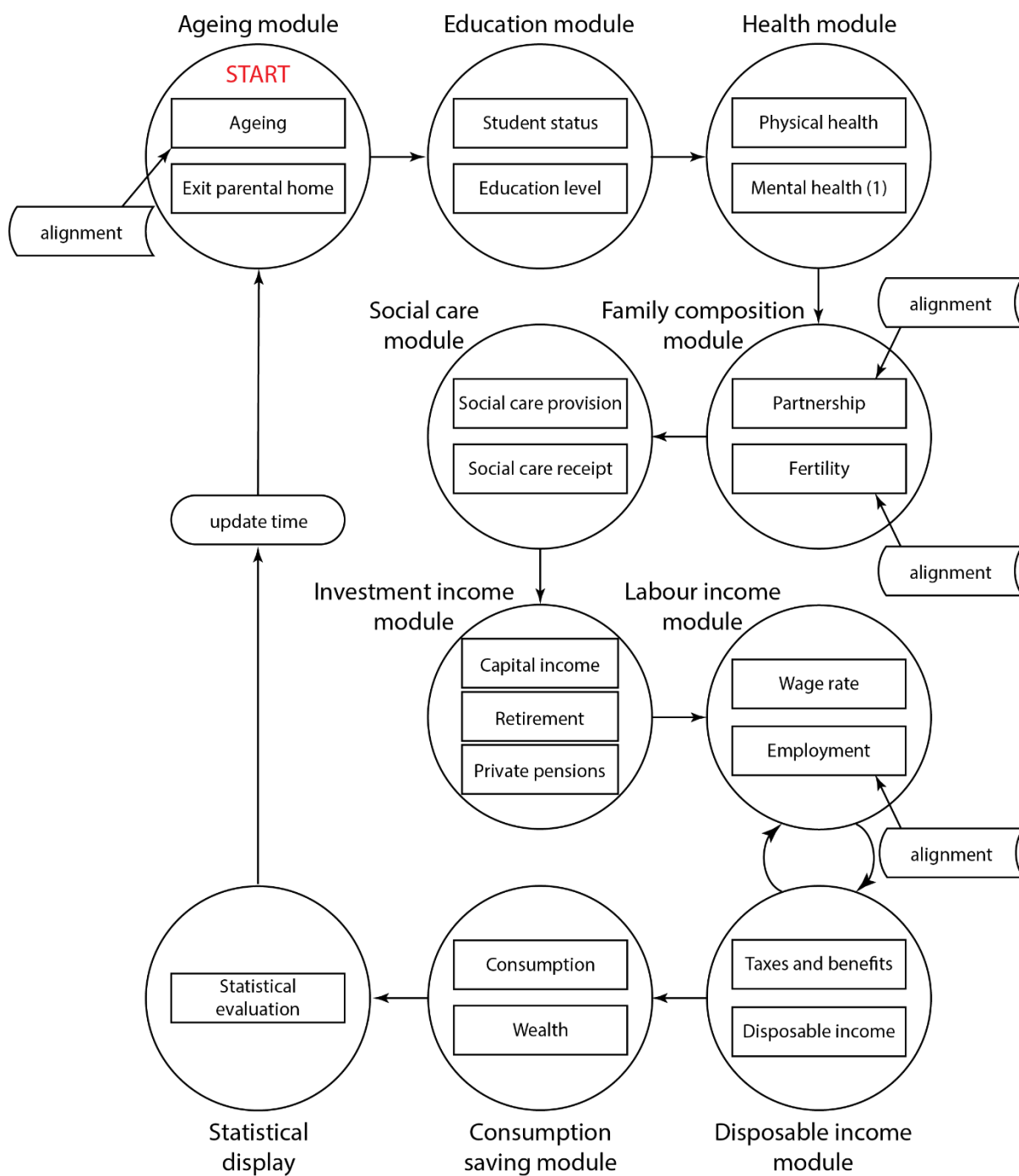
Figure 3.1: Module configuration of the SimPaths microsimulation model
