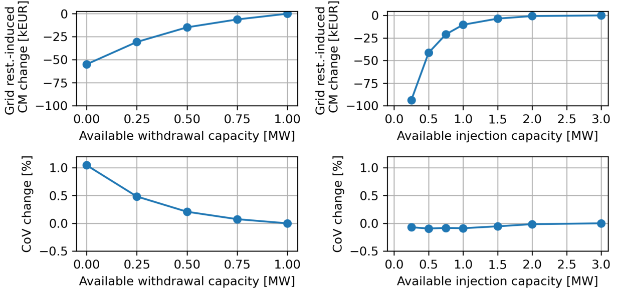
Figure 4: Grid restriction-induced contribution margin change and related changes in contribution margin variance.
