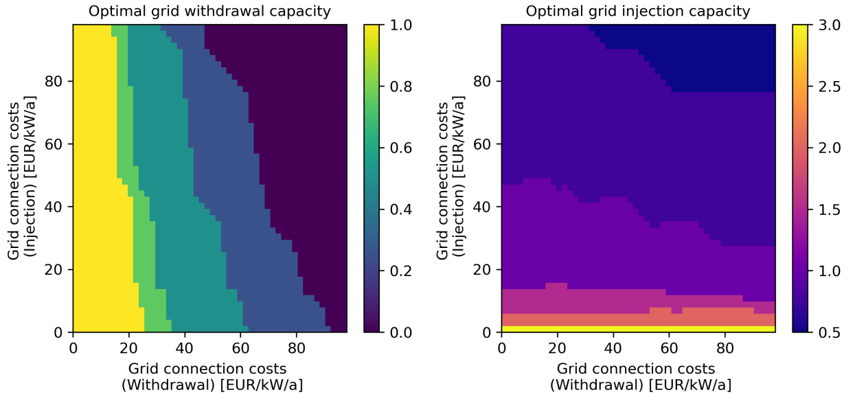
Figure E.9: Optimal grid connection configurations depending on the marginal grid connection costs.
