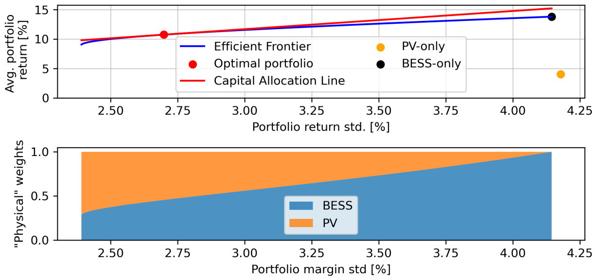
Figure C.8: Efficient frontier of hybrid PV-BESS system and analysis of respective weights.
