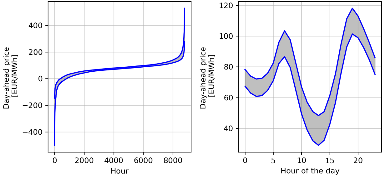
Figure 2: Price duration curve (left) and average hourly profile (right) of day-ahead price samples. The upper and lower limits of the samples are shown.
