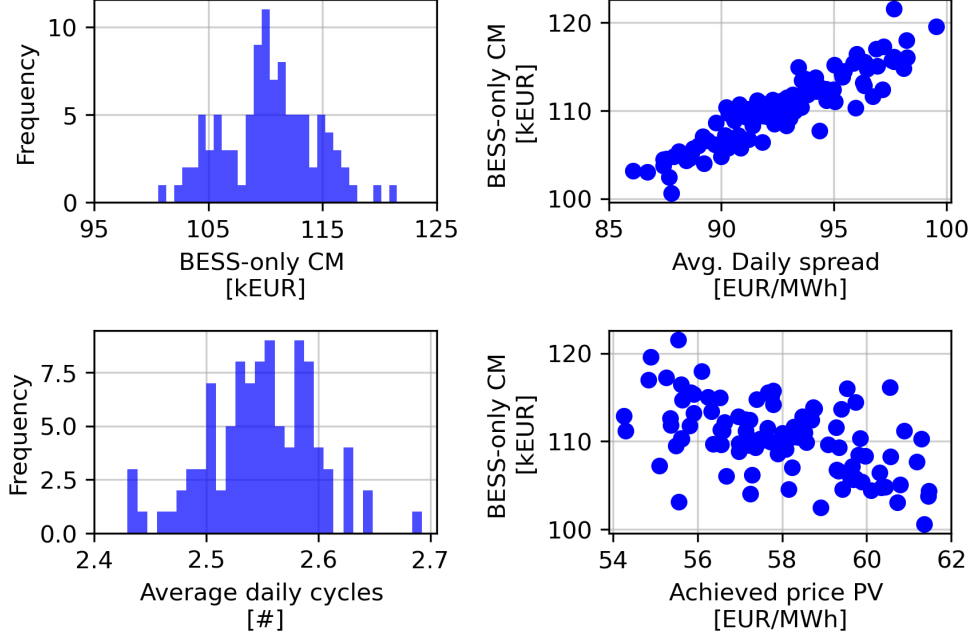
Figure 3: Distribution of margins and cycles in the base case, and relevant correlations.
