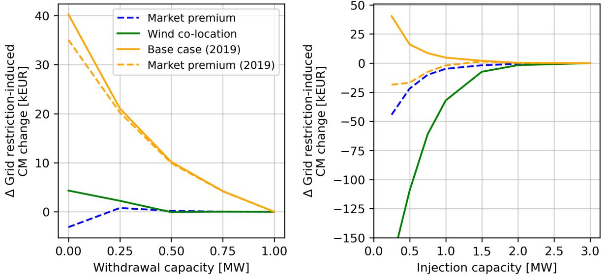
Figure 6: Difference in the grid restriction-induced contribution margin change relative to the base case for different scenarios (represented by the different lines).
