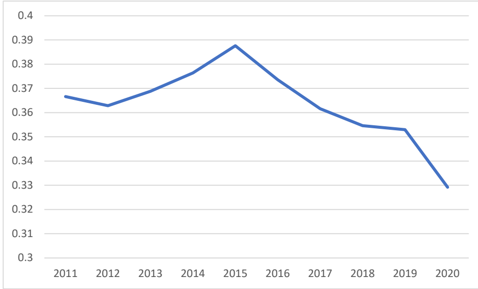
Figure 3. Average leverage by year.
