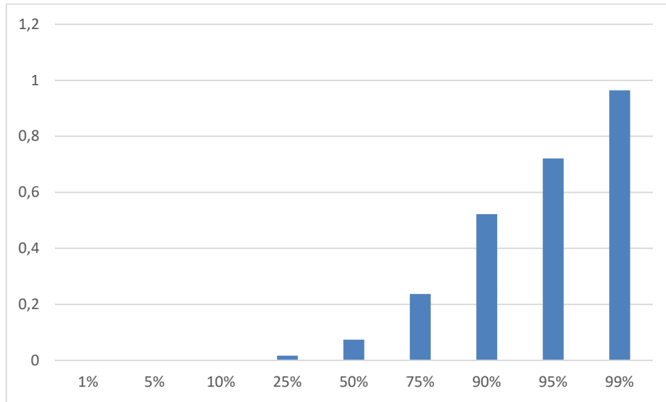
Figure 4. The mean of USNI by quantile.
