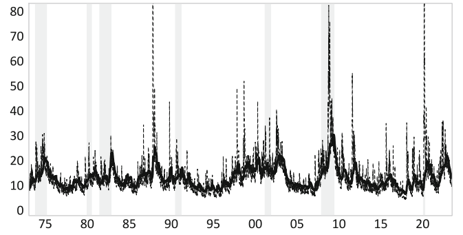
FIGURE 4 | The figure shows the estimated conditional volatility, \sqrt{h_t \tau_t} , (dashed line) and long-term volatility, \sqrt{\tau_t} , (solid line) from the MF2-GARCH-rw-63 model for the daily S&P 500 returns presented in Table 2. All quantities are annualized. Gray shaded areas represent NBER recession periods.
