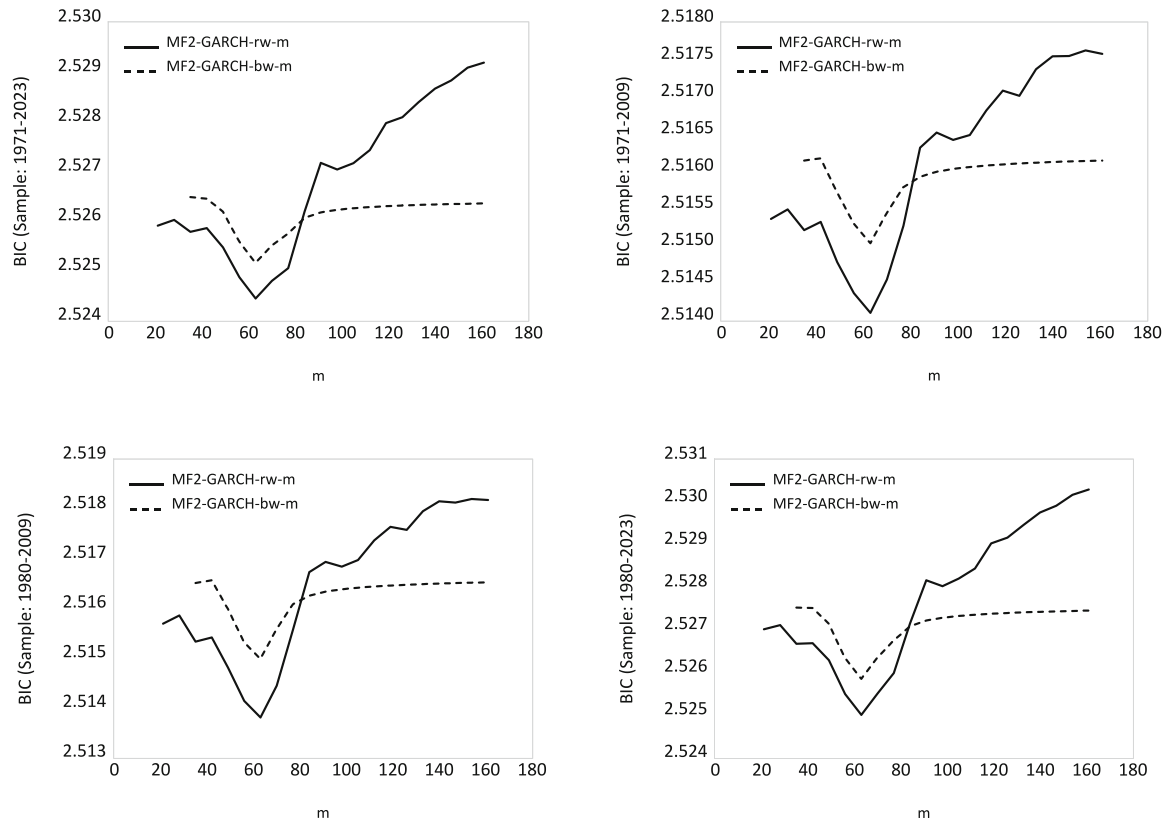
FIGURE 3 | MF2-GARCH-rw- m and MF2-GARCH-bw- m models are estimated using daily S&P 500 return data for the sample periods January 1971 to June 2023 (upper left), January 1971 to December 2009 (upper right), January 1980 to December 2009 (lower left), and January 1980 to June 2023 (lower right). The figure plots the BIC as a function of m .
