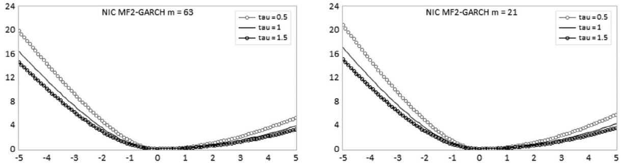
FIGURE 2 | The figure shows the NIC for an MF2-GARCH-rw- m model with m = 63 (left panel) and m = 21 (right panel) and parameters as in Figure A.3 in the Supporting Information. We fix h_t = 1 and assume that the short-term component correctly predicts volatility on days t - 1 to t - m - 1 , that is, we set r_{t-j}^2/h_{t-j} = 1 for j = 1, \dots, m - 1 . The NICs are plotted as a function of the return, r_t , and for \tau_t \in \{0.5, 1, 1.5\} . The NICs are standardized such that news impact is zero for r_t = 0 and presented as annualized volatilities, that is, we plot \sqrt{252(\sigma_{t+1}^2(r_t|\tau_t, h_t = 1) - \sigma_{t+1}^2(r_t = 0|\tau_t, h_t = 1))} .
