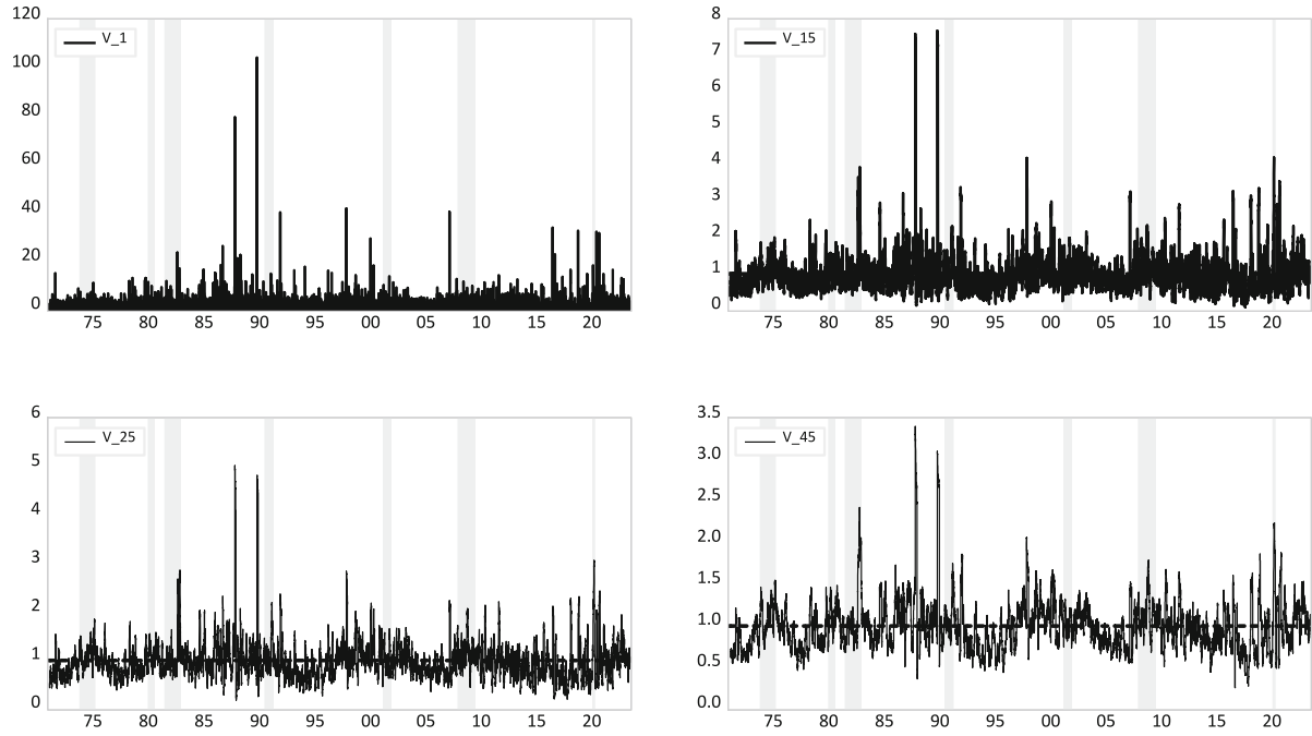
FIGURE 1 | A GJR-GARCH(1,1) is estimated for daily S&P 500 return data for the January 1971 to June 2023 period. The figure shows \tilde{V}_t^{(m)} for m = 1 (upper left panel), m = 15 (upper right panel), m = 25 (lower left panel), and m = 45 (lower right panel). Gray shaded areas represent NBER recession periods.
