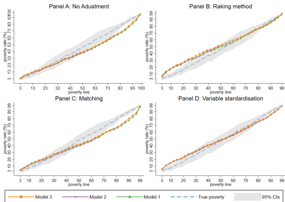
Fig. 1 Imputed income for different poverty lines based on ProGres19 using the model estimated from GEIH19, by variable transformation method Note: The blue dashed line offers the actual poverty rates derived from the GEIH survey, presenting poverty rates derived from observed income of the GEIH. The green solid curve with circle symbol represents the imputed poverty rates from Model 1 with observations from ProGres. The indigo solid curve with symbol “x” represents the imputed poverty rates from Model 2 using ProGres while the orange solid curve with the triangle symbol represents the imputed poverty rates from Model 3 using ProGres
