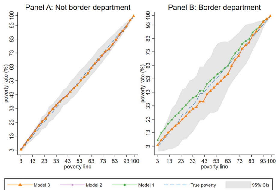
Fig. 21 Scenario 2—Non-border departments vs border departments Note: The blue dashed curve presents the actual poverty rates derived from the GEIH survey, meaning that the blue dashed curve presents poverty rates derived from observed income of the GEIH. The green solid curve with circle symbol represents the imputed poverty rates from Model 1 with observations from ProGres. The indigo solid curve with symbol “x” represents the imputed poverty rates from Model 2 with the ProGres while the orange solid curve with the triangle symbol represents the imputed poverty rates from Model 3 with the ProGres
