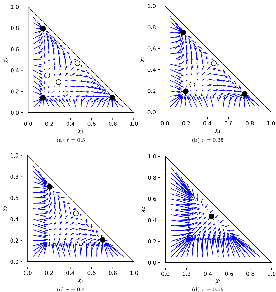
Fig. 5 The field G (see (9)) with A = 3 , \beta = 2 , \alpha_1 = \alpha_2 = \alpha_3 = 1 and \gamma = (0.4, 0.4, 0.2) for various labor shares r . Stable fixed points are marked with \bullet and unstable fixed points with \circ . Their exact position has been computed numerically with Mathematica
