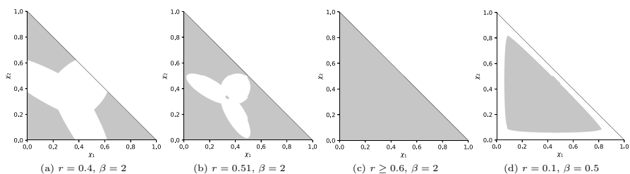
Fig. 17 The set P for A=3 and different r, \beta .
