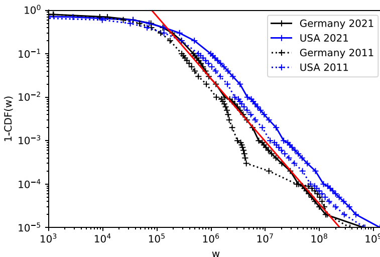
Fig. 1 1 - CDF (Cumulative Distribution Function) of net personal wealth (purchasing power parity, equal split adults) in Germany and the USA in 2011 and 2021 in Euro resp. US-Dollar according to World Inequality Database (2023). Least square fit (red line) estimates a Pareto exponent of 1.44 for Germany 2021 (colour figure online)
