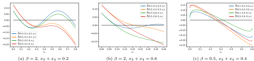
Fig. 18 The mapping \tilde{G}(r, x_3, x_4; x_1) := (1 - r) \frac{x_1^\beta}{x_1^\beta + (1 - x_1 - x_3 - x_4)^\beta + x_3^\beta + x_4^\beta} + 0.25r - x_1 for various parameterizations
