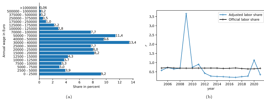
Fig. 6 a shows the distribution of annual net wages in Germany 2018 per taxpayer based on data from Statistisches Bundesamt (2018). b presents empirical values of the labor share r for several years in Germany computed according to formula (17) using data from WID (2023) and Statistisches Bundesamt (2022) compared to the official labor share from Bundesfinanzministerium (2022)
