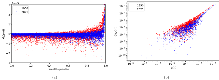
Fig. 20 Scatter plot of G_i(\chi(n)) against wealth quantiles (a) and against \chi_i(n) for positive G_i only (b), for the years 1950 and 2021 in our simulation with symmetric initial condition. Years were assigned via (18) assuming a constant growth rate of \mu = 0.03 per year. The entries of the field G slowly tend to zero asymptotically and this happens faster for poorer agents (cf. Sect. 4.5)
