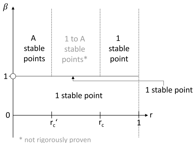
Fig. 2 Qualitative illustration of the number of stable fixed points of G for feedback of the form F_i(k) = \alpha_i k^\beta depending on labor share r and reinforcement parameter \beta . \circ marks the classical Pólya urn, which exhibits either deterministic (weak) monopoly or a Dirichlet distributed limit
