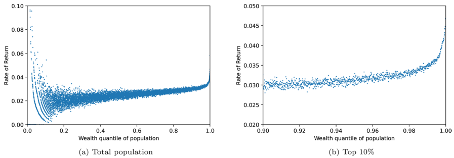
Fig. 10 Rate of Return on capital between step n = 216,000,000 and n = 228,000,000 in the Pareto case plotted against wealth quantiles. This corresponds to the year 2020
