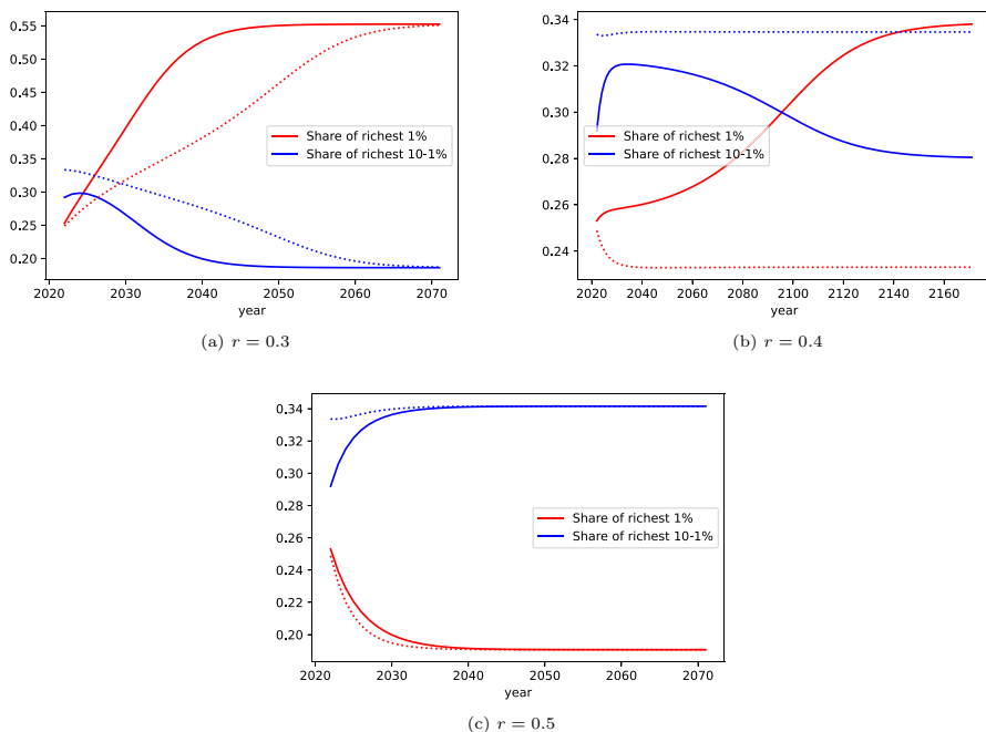
Fig. 16 Evolution of the wealth share of the richest 1% (red) and the following 9% (blue) in the solution of (19) for different labour shares r . We used x_{ger} (after normalization and fully correlated with \gamma , full line) and the result from the simulation with X(0) = (1, \dots, 1) (dotted line) as initial condition. Note the different scales on the axes (colour figure online)
