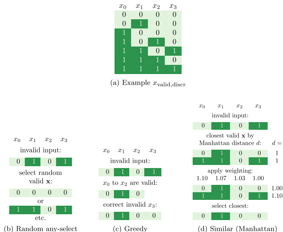
Fig. 3 A visualization of different eager correction strategies
