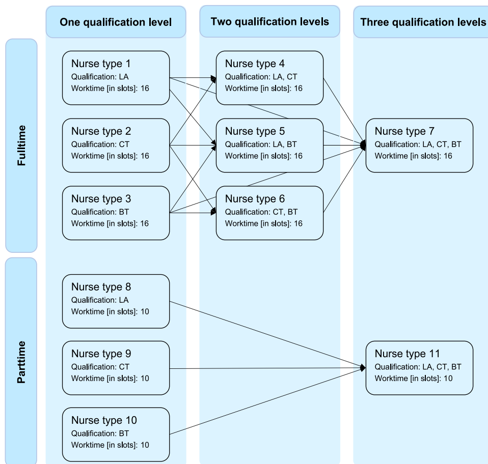
Fig. 4 Qualification level connection between the different nurse types
