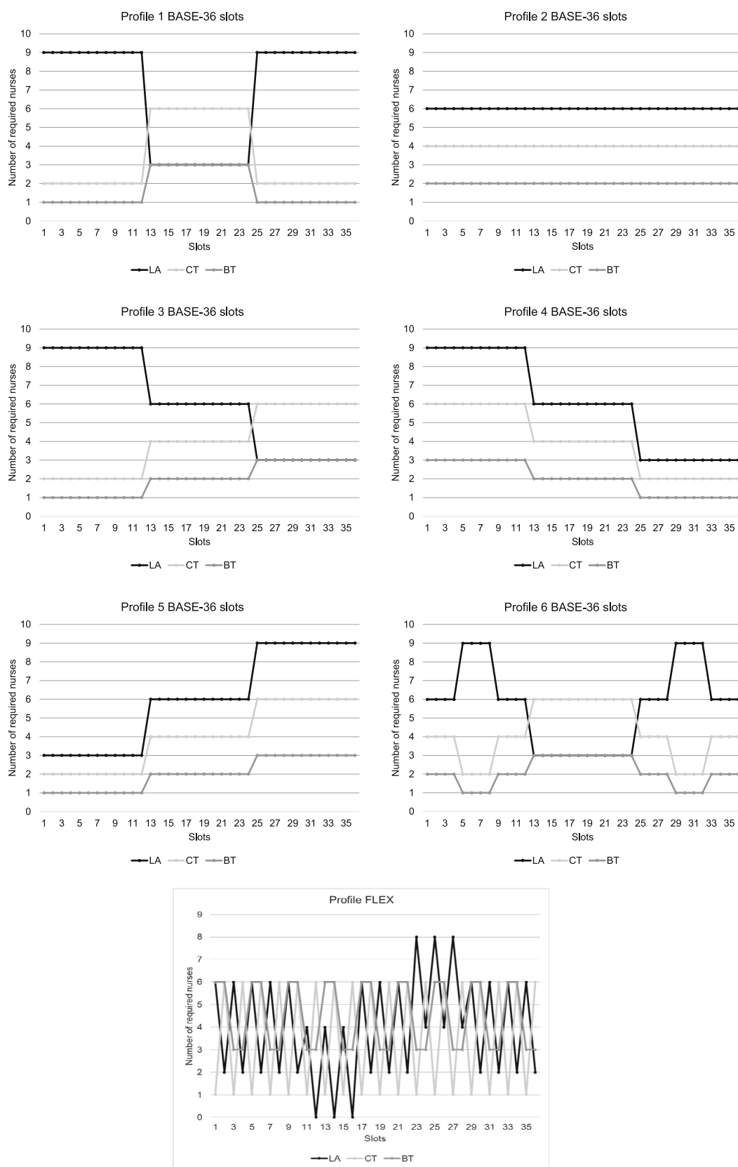
Fig. 7 Different demand profiles
