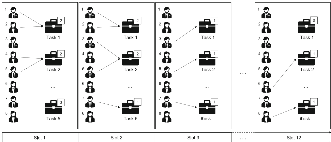
Fig. 2 Visualization for 8 workers, 5 tasks, and 12 time slots
