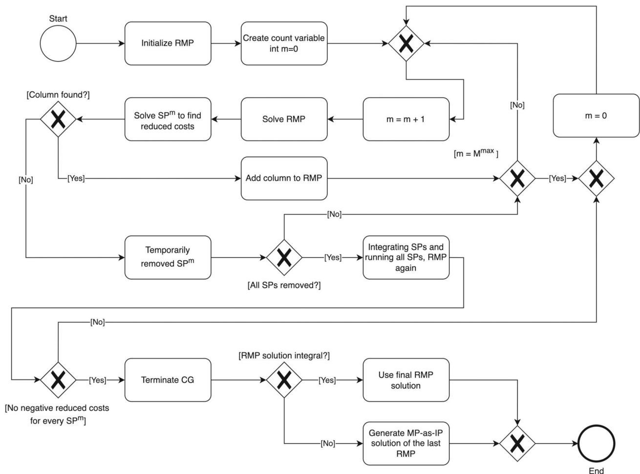
Fig. 3 Column generation (CG) algorithm process flow
