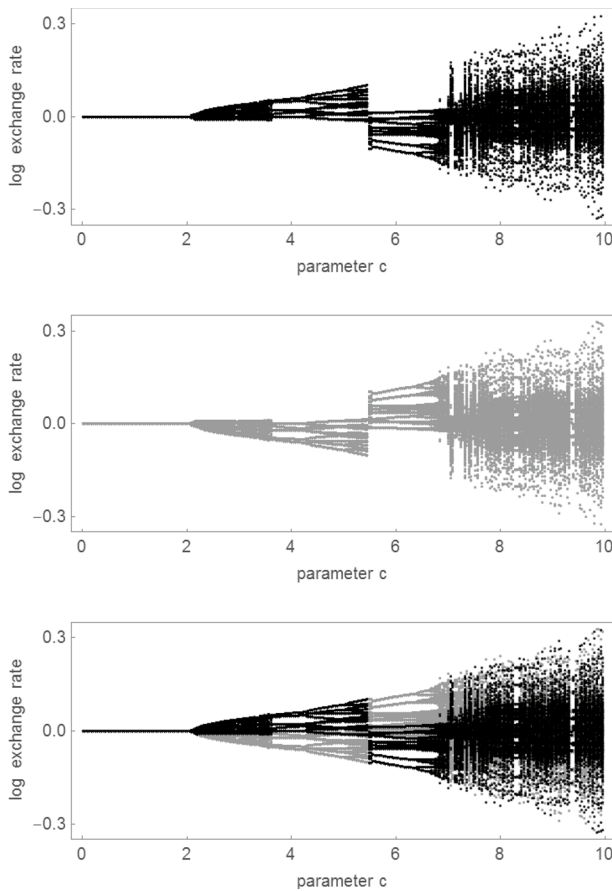
Fig. 4 Parameter c . The first two panels depict bifurcation diagrams in which the log exchange rate is portrayed as a function of parameter c for two different sets of initial conditions, given by S_0 = 0.01 , X_0 = 0 , Y_0 = 0 and S_0 = -0.01 , X_0 = 0 , Y_0 = 0 , respectively. The third panel displays both bifurcation diagrams. Remaining parameters: F = 0 , m = 1 , N = 1 , f = 0.3 , s_0 = 0.05 and s_1 = 2500
