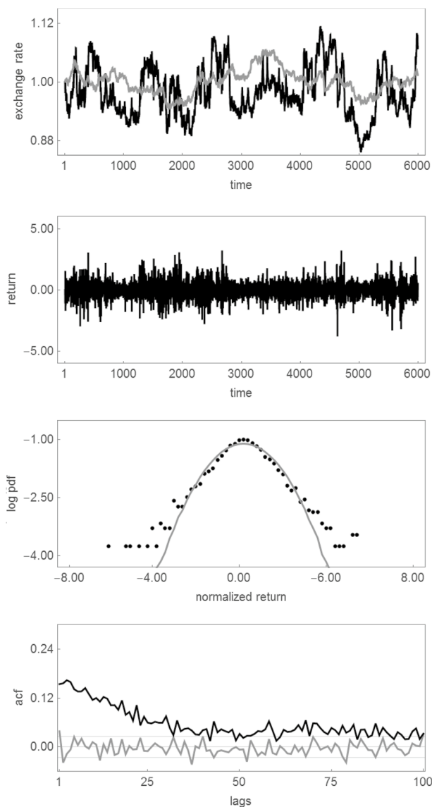
Fig. 8 Simulation run #3. The first panel shows the evolution of simulated exchange rates (black line) and their fundamental values (gray line) for 6000 observations. The second panel shows the corresponding return dynamics. The third panel shows the log probability density function of normalized returns. The fourth panel shows autocorrelation functions of raw returns (gray line) and absolute returns (black line)
