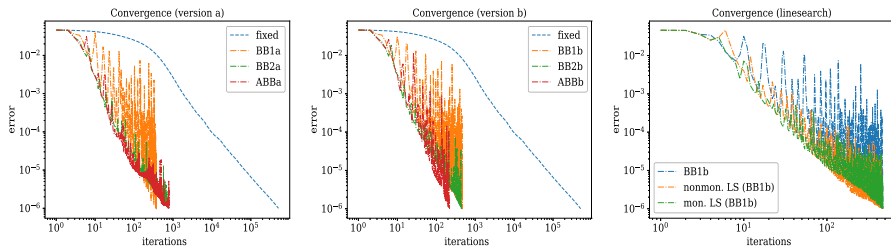
Fig. 7 Example 2: convergence of Algorithm 1. “Error” refers to \|\mathcal{G}_{\alpha_k}(u_k)\|_H at the current iterate
