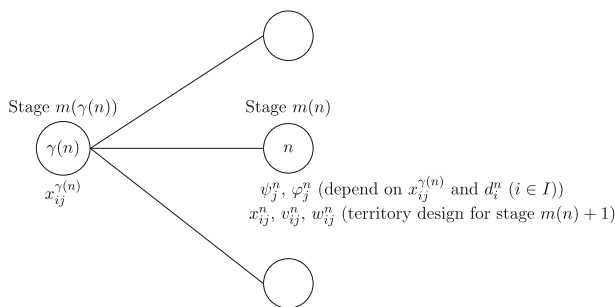
Fig. 2 Illustration of the building blocks for Constraints (19)
