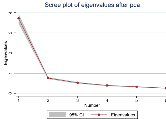
Figure A13: Eigenvalues after Principal Component Analysis
