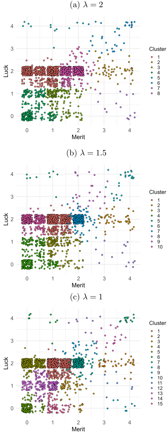
Figure C7: DP-Means Clustering
