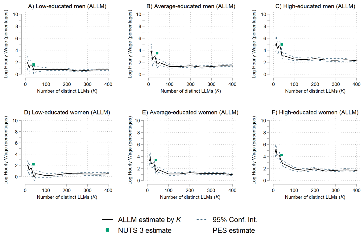
Fig. B.3. Aggregate LLM UWP by subgroups based on the OLS two-step procedure (Eq. (B.2)).
