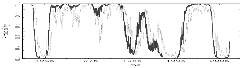
(a) Ex ante and smoothed probabilities
