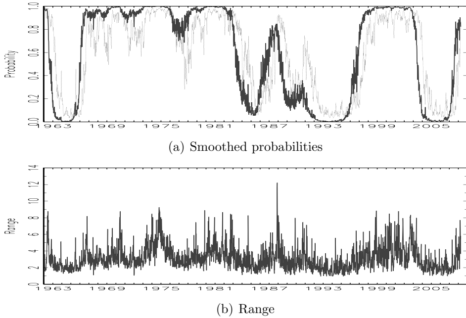
Figure 6: S&P500 range and smoothed probabilities
