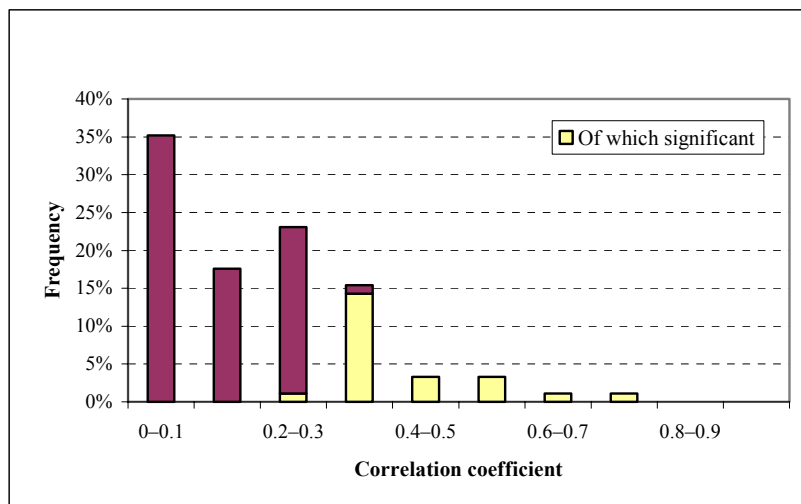
Figure 4. Frequency distribution of correlation coefficients between indicators
