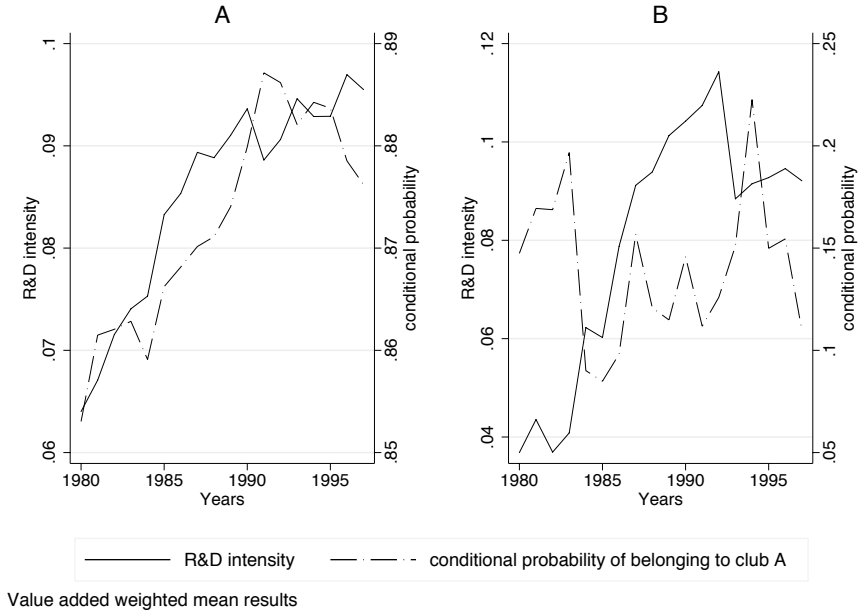
Figure 1. R&D intensity and conditional probability of belonging to club A
