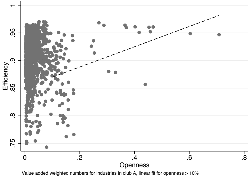
Figure 3. Efficiency and openness to trade
