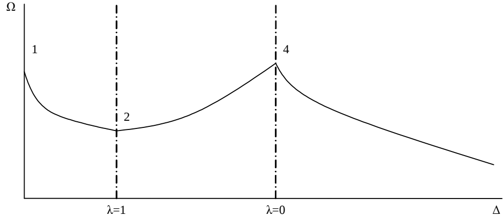
Figure 2: No local minimum for 0 < \lambda < 1
