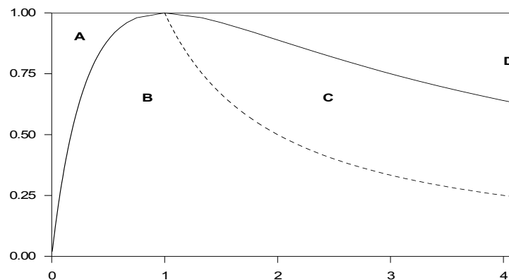
Figure 1: Diagram showing boundaries of regions yielding different qualitative behaviour (Adapted from Samuelson, 1939: 78. Vertical axis: \alpha = marginal propensity to consume. Horizontal axis: \beta = accelerator coefficient)
