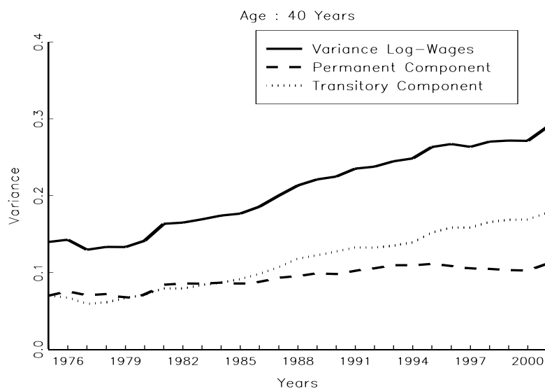
Figure 4: The estimated variances of the transitory and permanent components of log-wages over the period 1975-2001.
