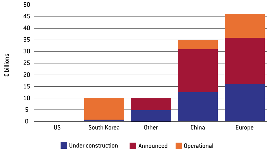
Figure 2: Battery investment in Europe by source, 2020-2024
