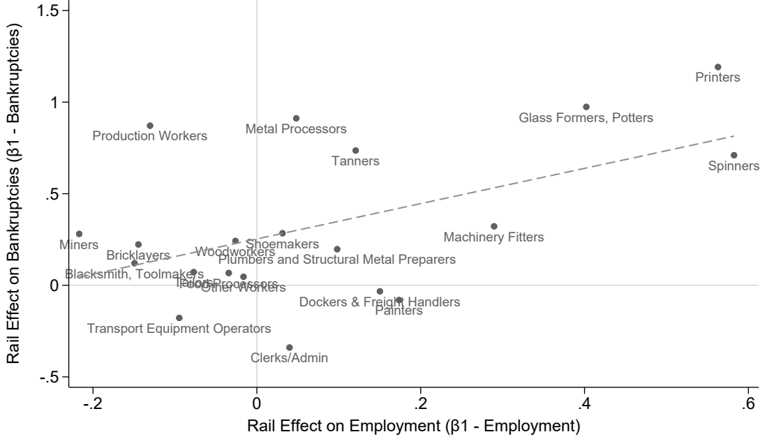
Figure 4: Within-Manufacturing estimates
