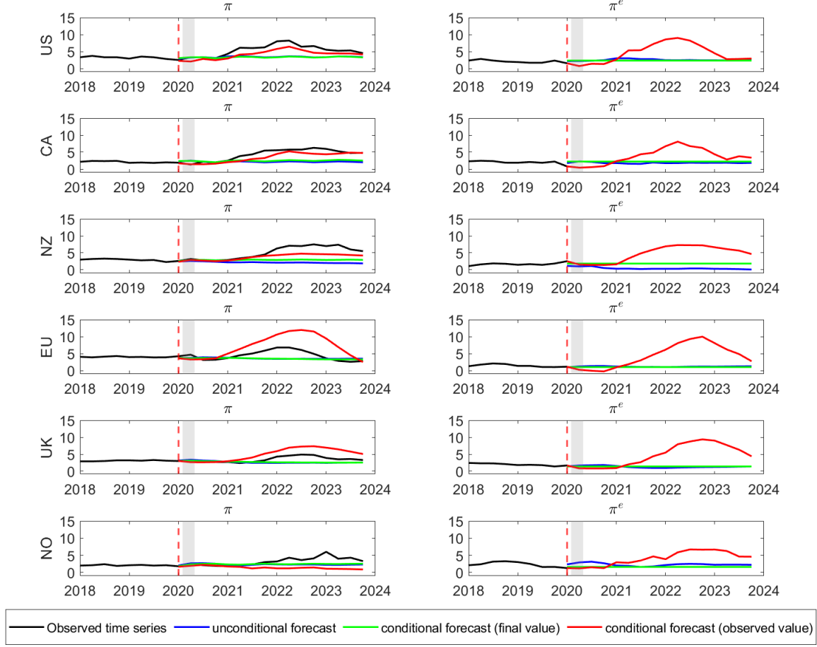
Figure 7: Conditional Forecasts. The countries under study are the US, Canada (CA), New Zealand (NZ), the Euro area (EU), the UK and Norway (NO).
