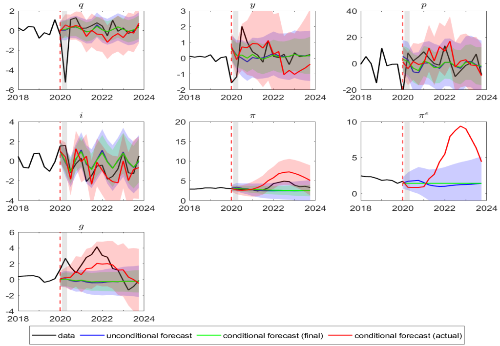
Figure 23: UK: Conditional forecasts in the pandemic period.
