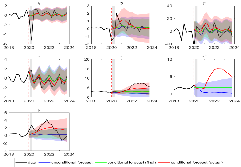
Figure 21: New Zealand: Conditional forecasts in the pandemic period.
