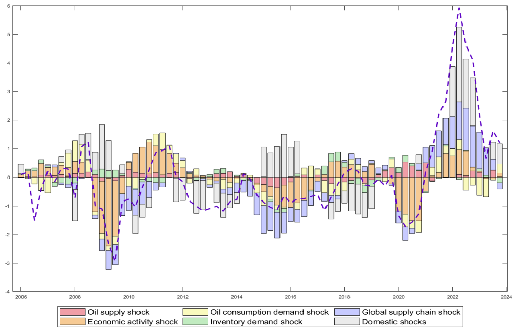
Figure 14: Canada: Historical decomposition for CPI (demeaned) full sample
