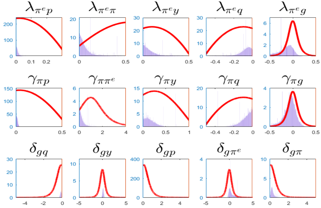
Figure 9: New Zealand: Prior (solid red curves) and posterior (purple histograms) distributions of structural parameters in the inflation and GSCPI blocks.
