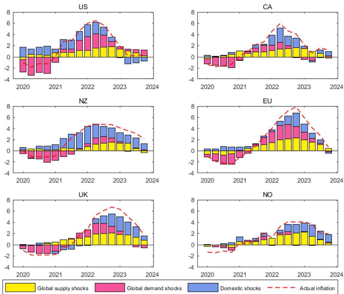
Figure 5: Historical Decomposition CPI (demeaned) from 2020. The countries under study are the US, Canada (CA), New Zealand (NZ), the Euro area (EU), the UK and Norway (NO).
