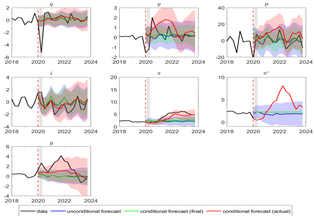
Figure 20: Canada: Conditional forecasts in the pandemic period.
