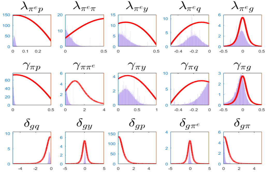
Figure 12: Norway: Prior (solid red curves) and posterior (purple histograms) distributions of structural parameters in the inflation and GSCPI blocks.
