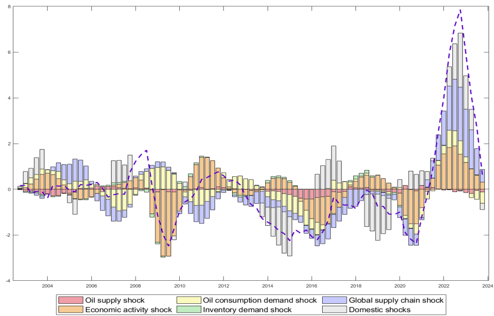
Figure 16: Euro area: Historical decomposition for CPI (demeaned) full sample
