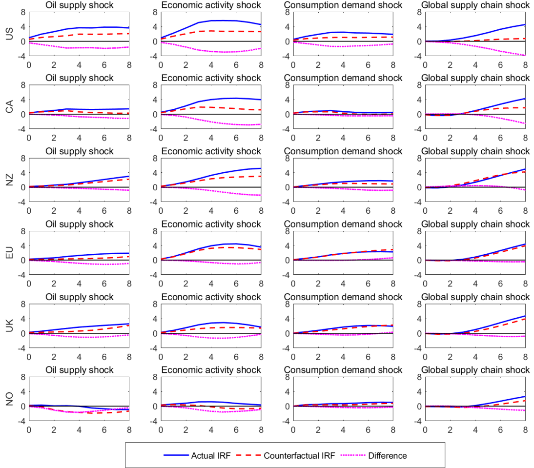
Figure 4: Actual and counterfactual: Holding inflation expectations constant. The countries under study are the US, Canada (CA), New Zealand (NZ), the Euro area (EU), the UK and Norway (NO).
