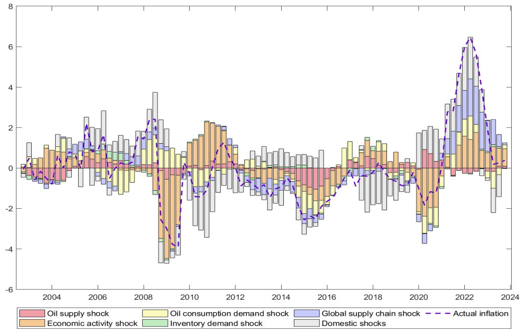
Figure 13: US: Historical decomposition for CPI (demeaned) full sample
