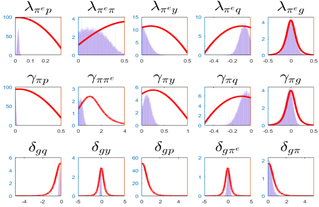
Figure 11: UK: Prior (solid red curves) and posterior (purple histograms) distributions of structural parameters in the inflation and GSCPI blocks.
