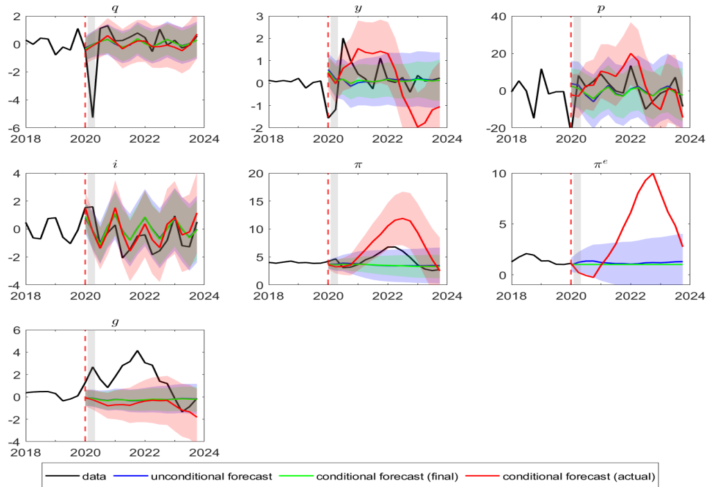
Figure 22: Euro area: Conditional forecasts in the pandemic period.
