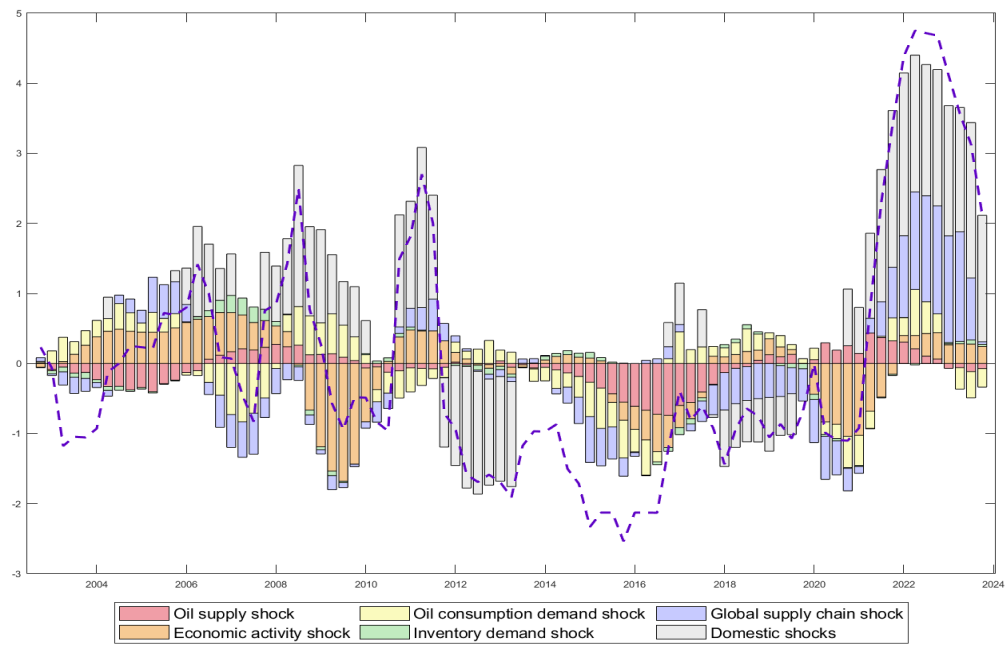
Figure 15: New Zealand: Historical decomposition for CPI (demeaned) full sample
