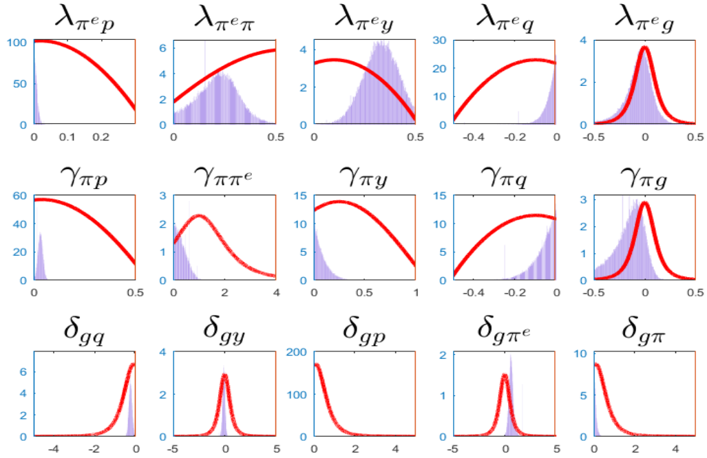
Figure 8: Canada: Prior (solid red curves) and posterior (purple histograms) distributions of structural parameters in the inflation and GSCPI blocks.
