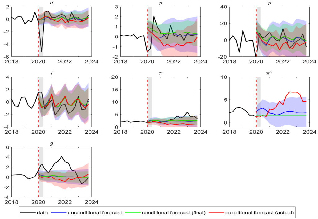
Figure 24: Norway: Conditional forecasts in the pandemic period.
