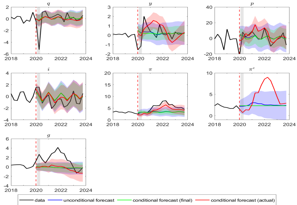
Figure 19: US: Conditional forecasts in the pandemic period.
