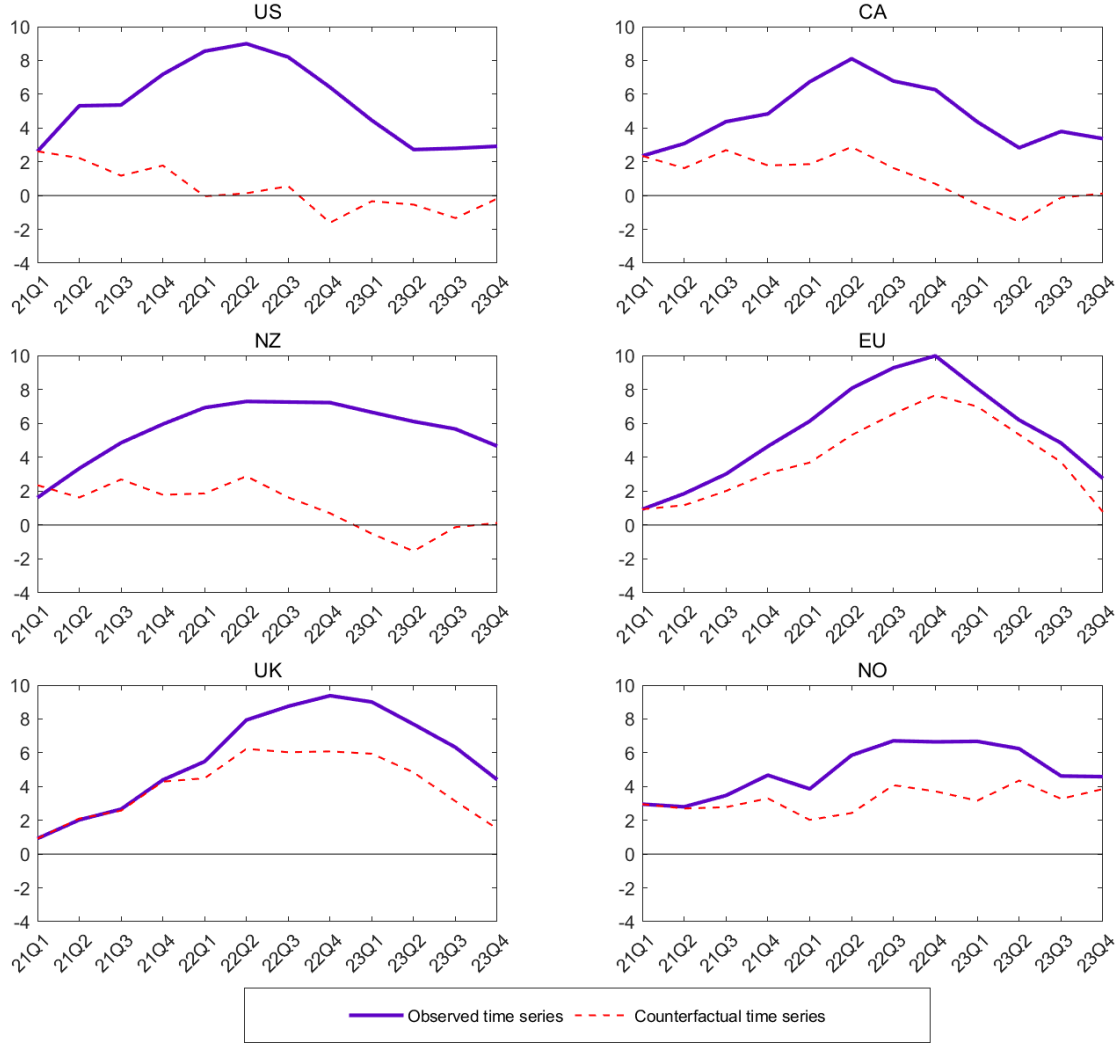
Figure 6: Counterfactual exercise - holding inflation expectations constant from 2021Q1. The countries under study are the US, Canada (CA), New Zealand (NZ), the Euro area (EU), the UK and Norway (NO).
