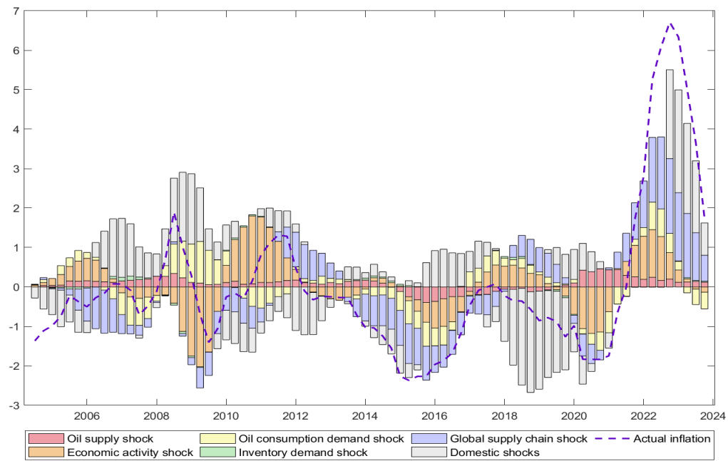
Figure 17: UK: Historical decomposition for CPI (demeaned) full sample
