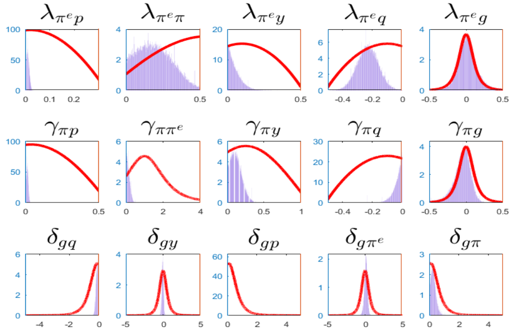
Figure 10: Euro area: Prior (solid red curves) and posterior (purple histograms) distributions of structural parameters in the inflation and GSCPI blocks.
