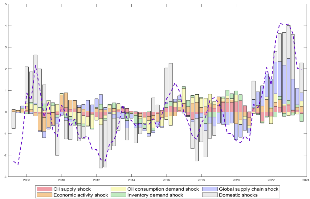
Figure 18: Norway: Historical decomposition for CPI (demeaned) full sample
