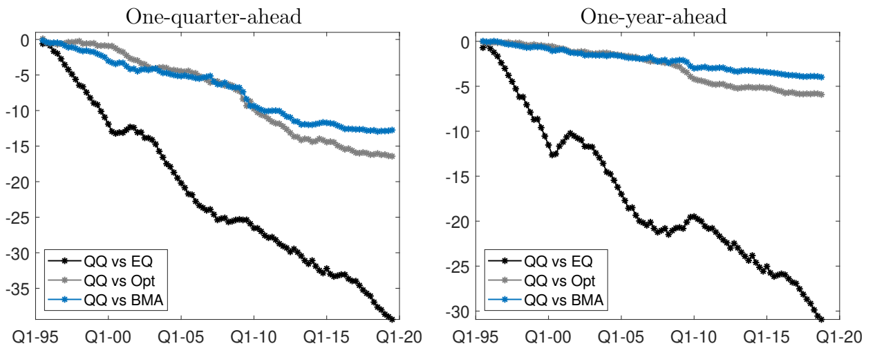
Figure 1: Cumulative CRPS of alternative combination approaches relative to the quantile combination for one-quarter and one-year ahead forecasts.
