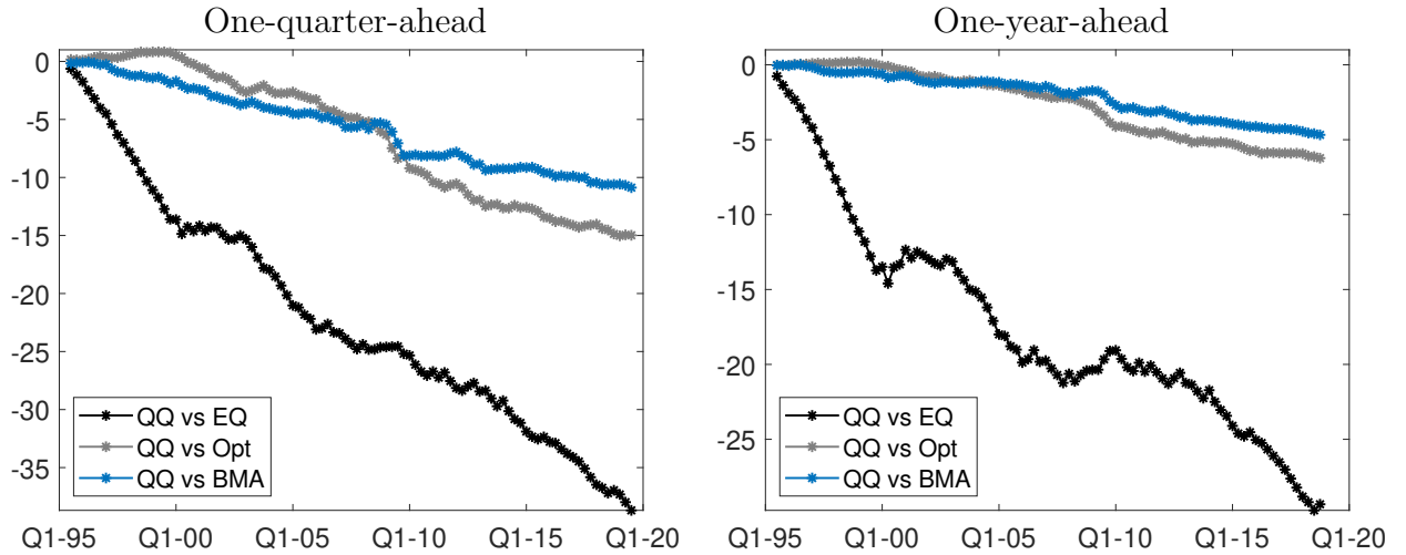
Figure A.5: Cumulative CRPS of the alternative combination approaches relative to quantile combination for one-quarter and one-year ahead forecasts - quantiles fitted on a non-parametric distribution.
