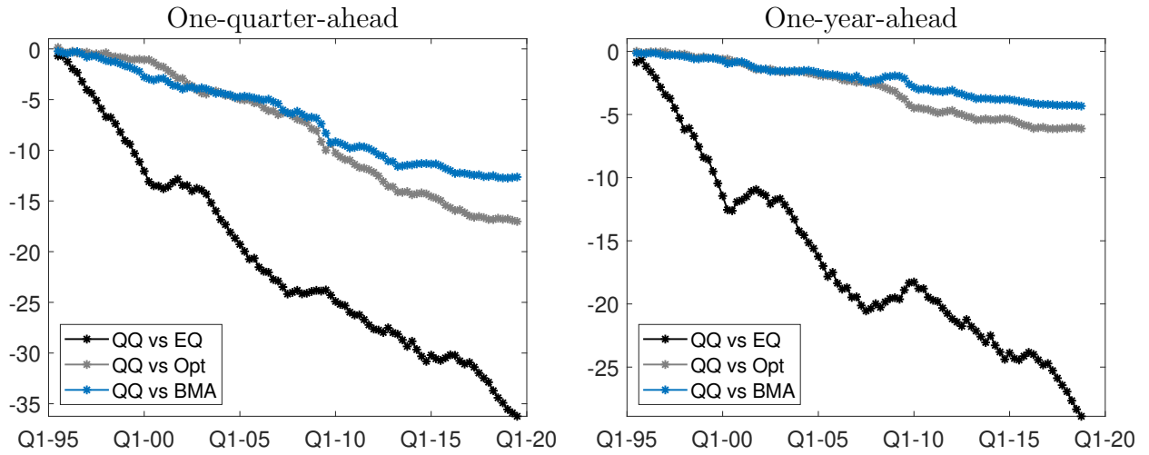
Figure A.13: Cumulative CRPS of the alternative combination approaches relative to quantile combination for one-quarter and one-year ahead forecasts - first release of GDP.
