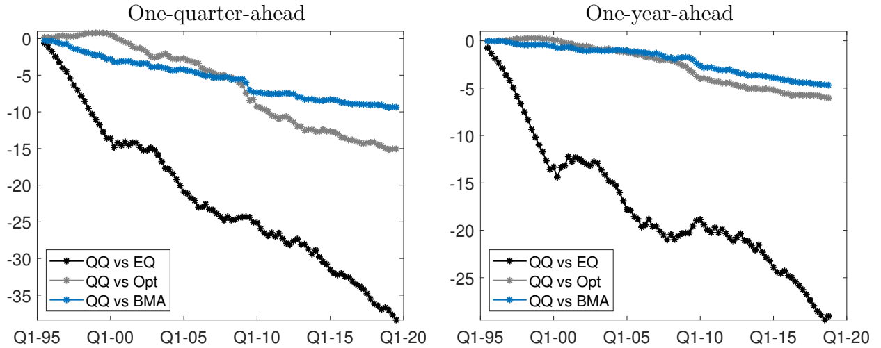
Figure A.17: Cumulative CRPS of the alternative combination approaches relative to quantile combination for one-quarter and one-year ahead forecasts - latest available release of GDP.
