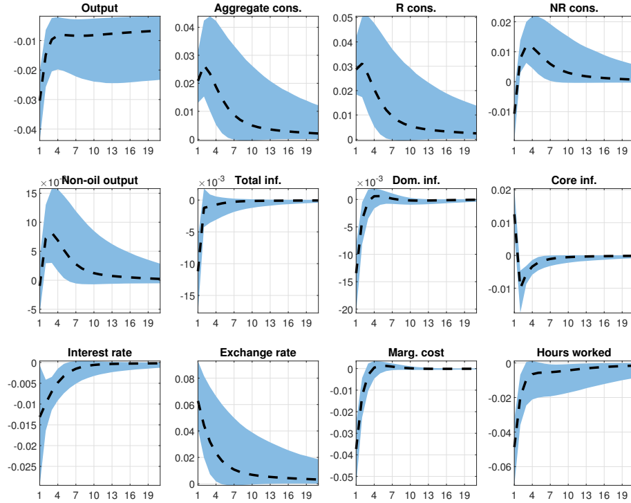
Figure 10: Responses to a Negative Oil Price Shock with s_2 and \nu = 1
