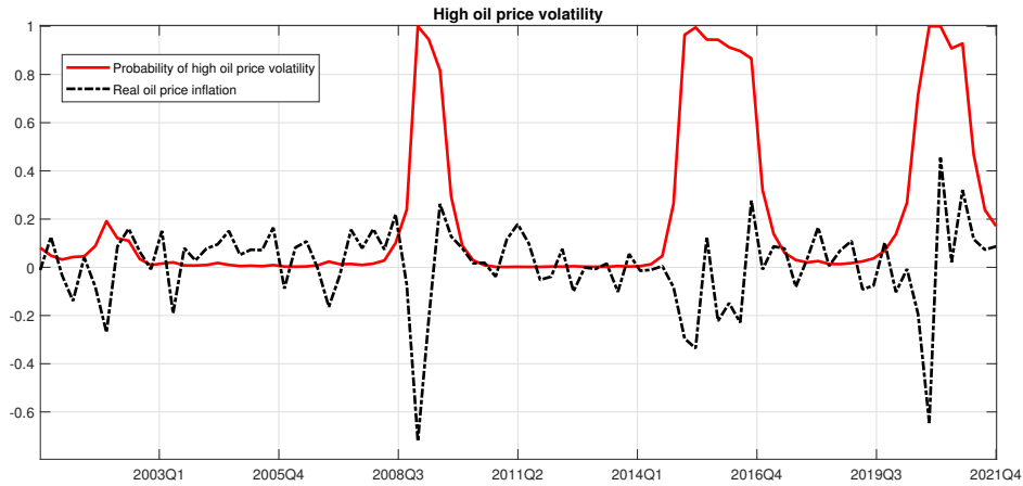
Figure 1: Smoothed Probability of High Volatility Regime ( s_2 )
