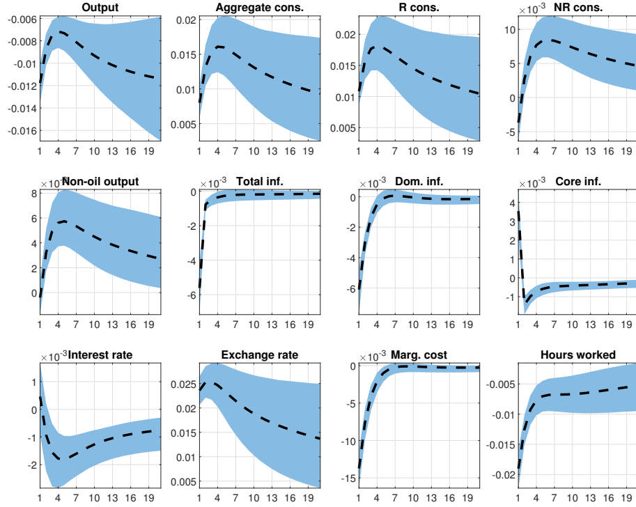
Figure 9: Responses to a Negative Oil Price Shock with s_1 and \nu = 1
