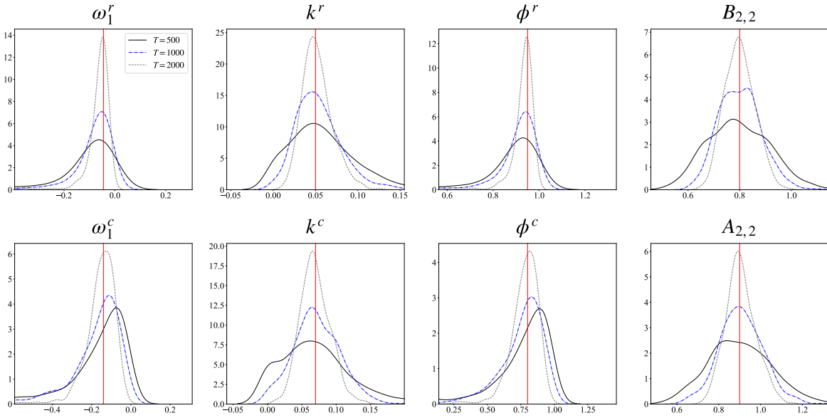
Figure 2: Kernel density estimates of the estimated parameters from 500 simulations for three sample sizes ( T = 500, 1000, 2000 ) are presented, with vertical red lines indicating the true parameter values.
