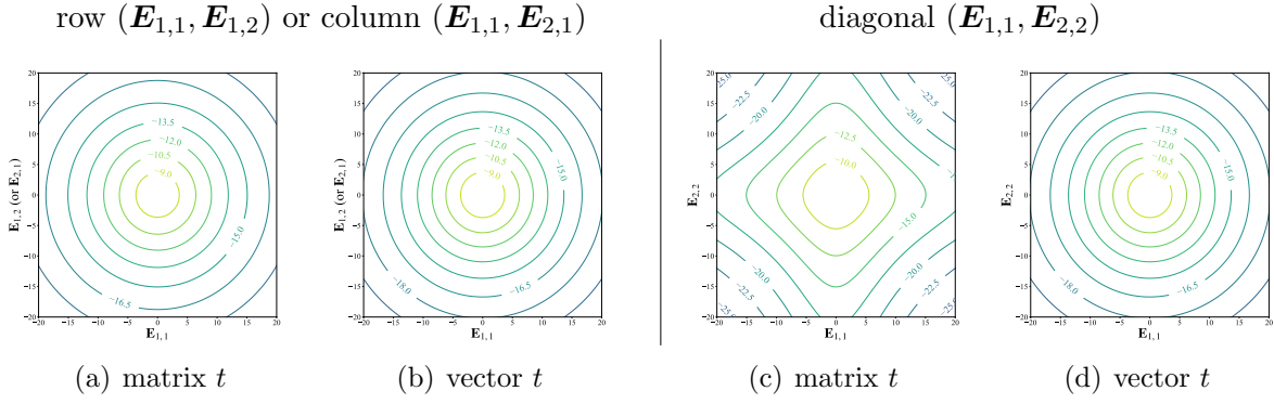
Figure 1: Log-pdf contour plots for the matrix and vector-valued t distribution
