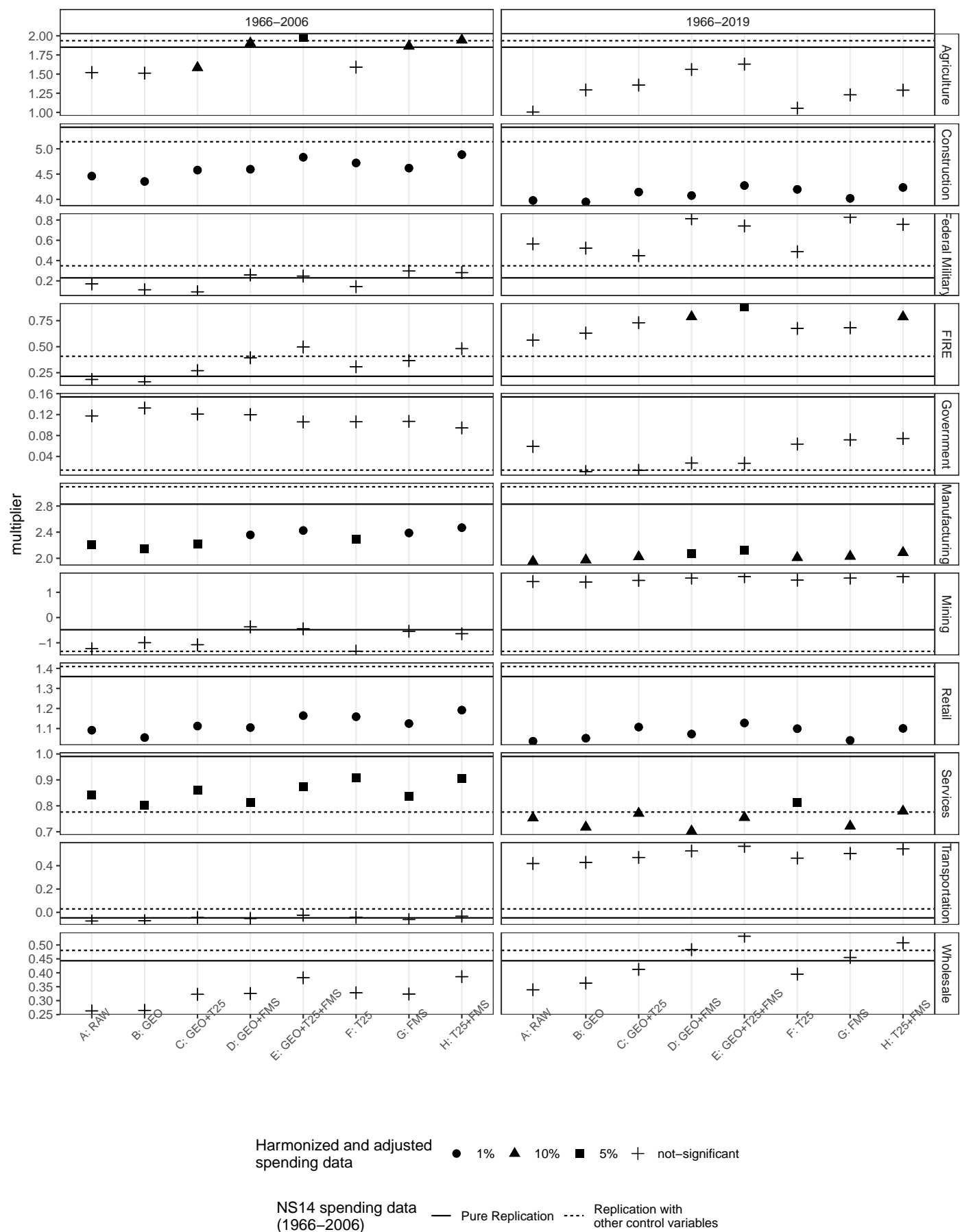
Figure 4: Revisited estimates of cross-sectional (state-level) fiscal spending sectoral output multipliers
