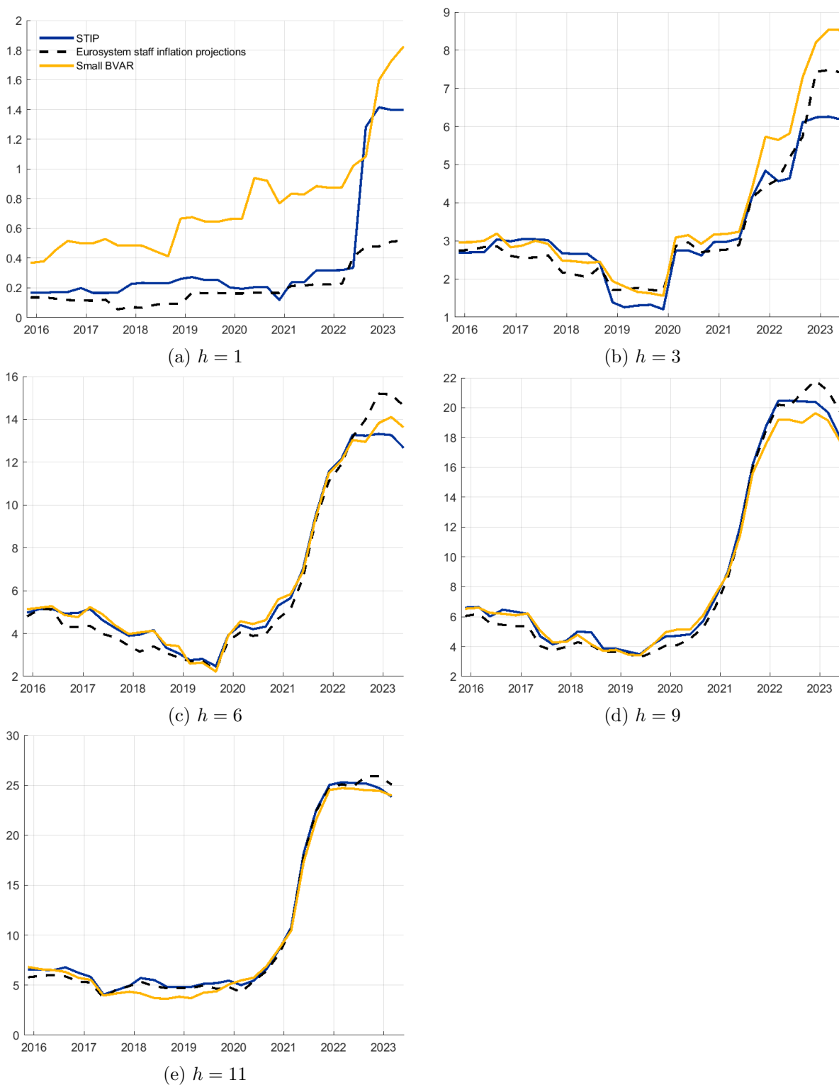
Figure 10: Rolling RMSFE: Model forecasts conditional on (B)MPE assumptions compared to the Eurosystem staff inflation projections.
