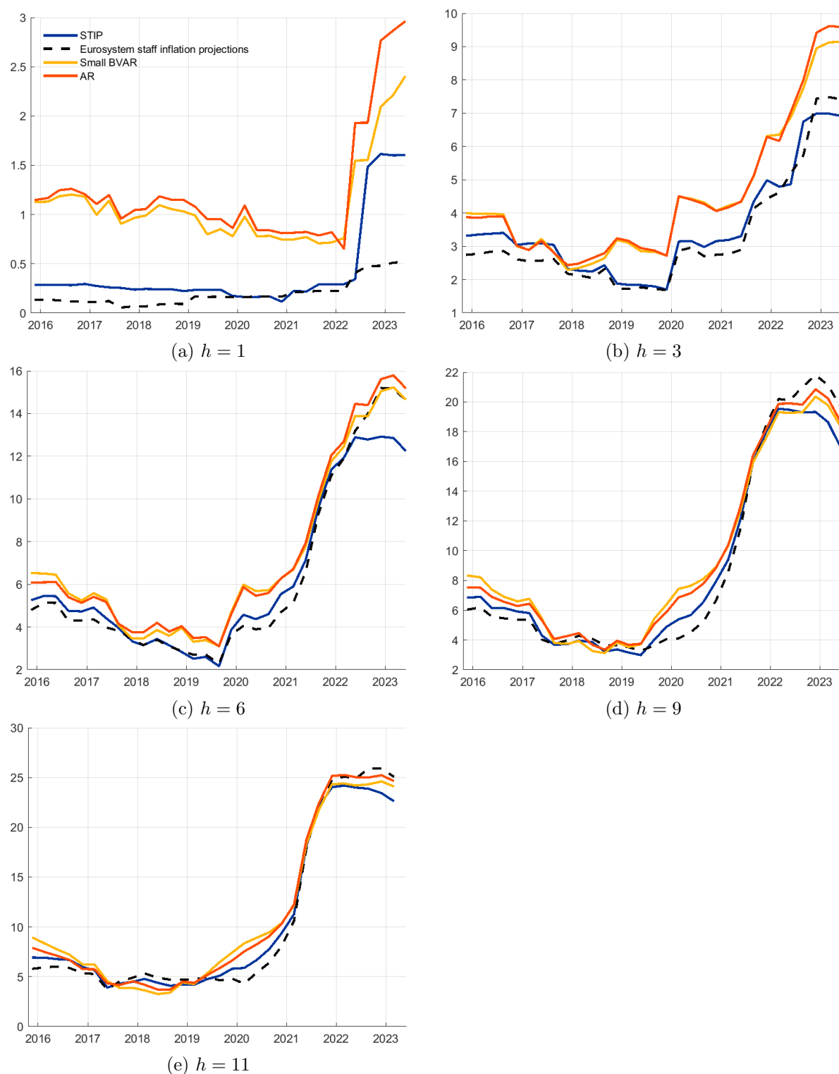
Figure 9: Rolling RMSFE: Unconditional model forecasts compared to the Eurosystem staff inflation projections.
