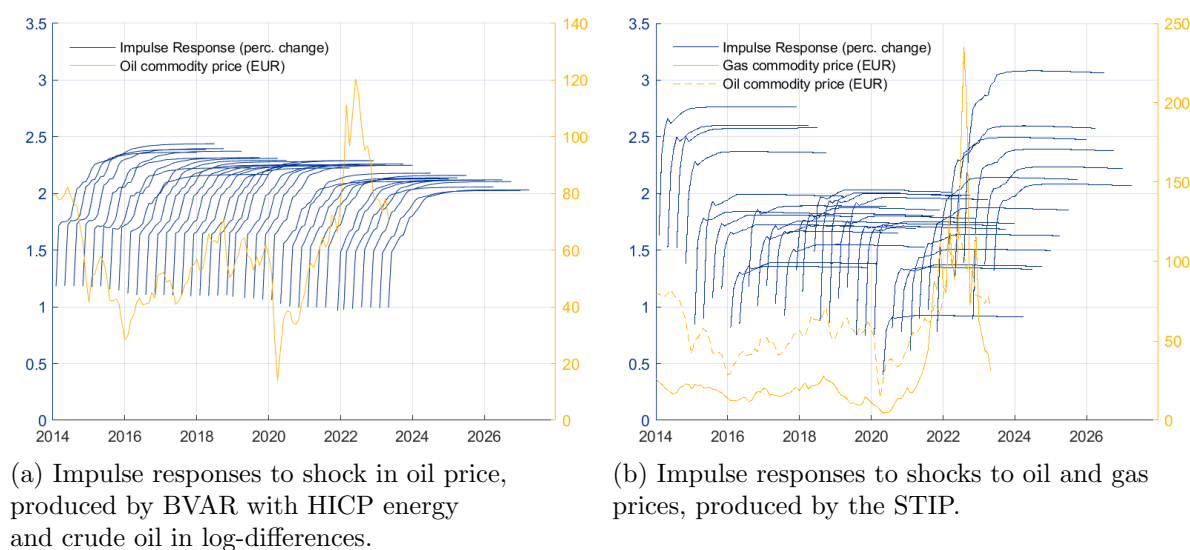
Figure 14: HICP energy response to 10% permanent shocks: BVAR vs STIP
