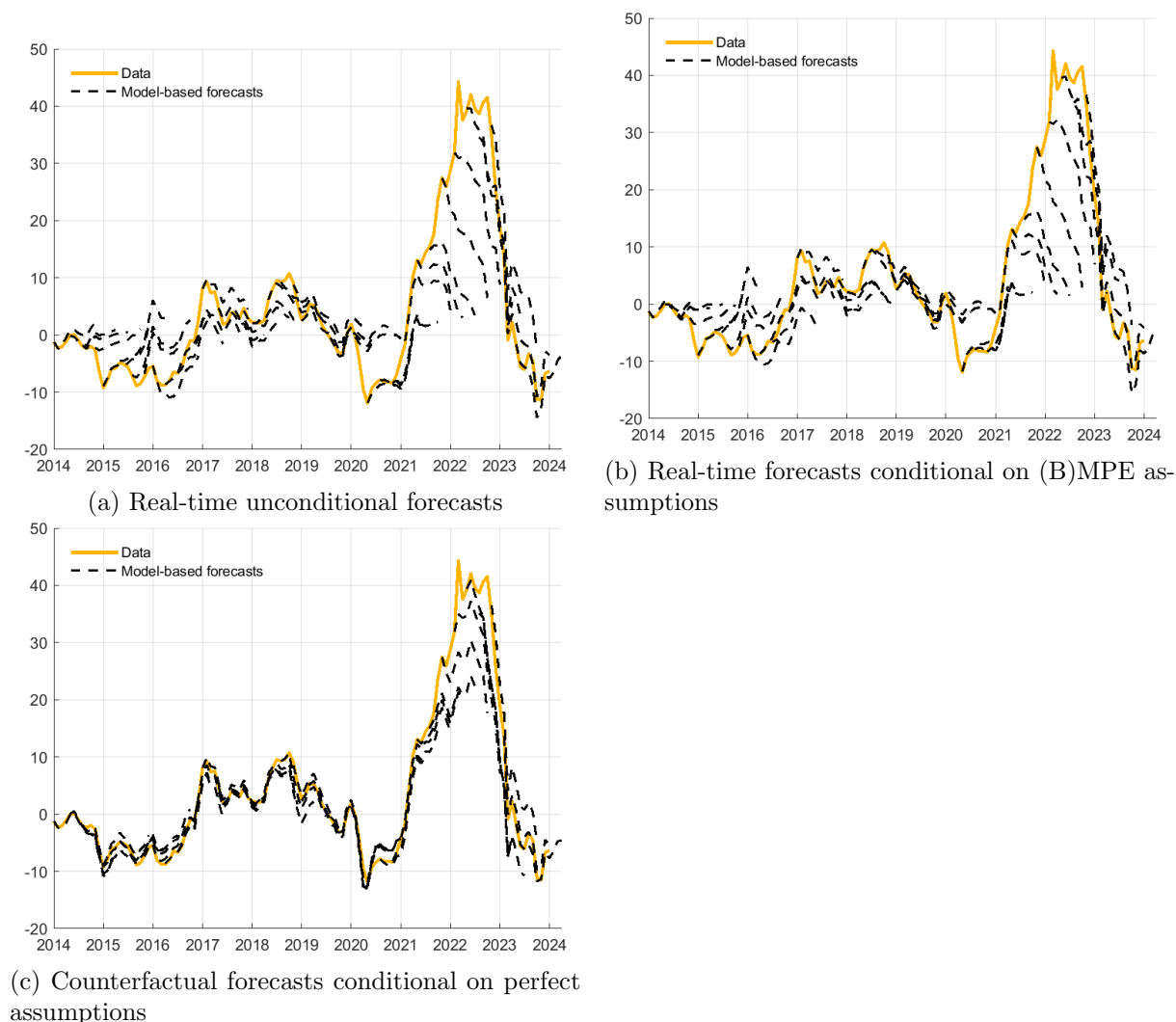
Figure 5: HICP energy real-time and counterfactual forecasts
