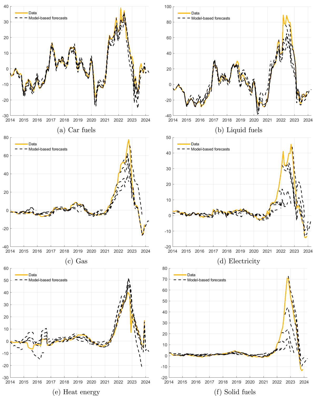
Figure 8: Counterfactual forecasts conditional on perfect assumptions
