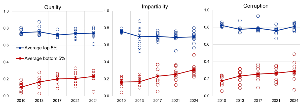
Figure A.2: EQI sub-components: developments over time of top 5% and bottom 5% regions in 2010
