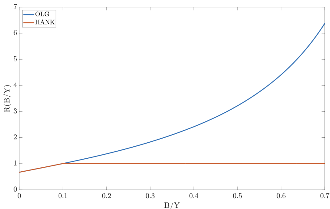
Figure 4: Steady-State R(B/Y) Relationship, HANK vs. OLG
