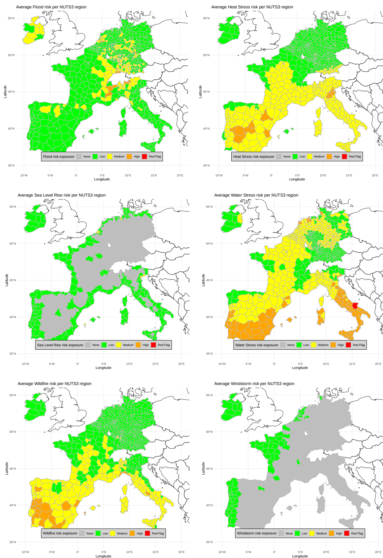
Figure 6: Risk of various physical climate risks per NUTS3 region.
